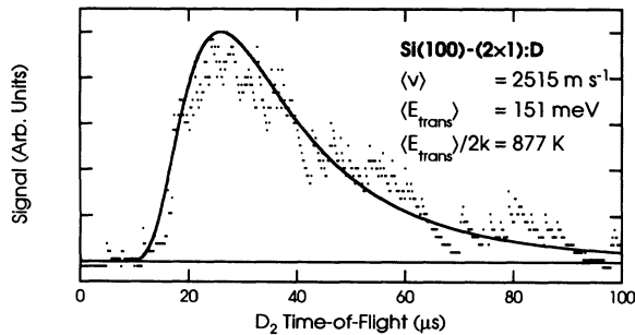
FIG. 1. TOF spectrum for D_2 thermally desorbed from the monohydride phase on Si(100)-(2 \times 1) with T_{\text{max}}=920 K. The dots represent the raw data (averaged over 256 laser shots) while the solid curve represents a fit by a Maxwell-Boltzmann distribution.
