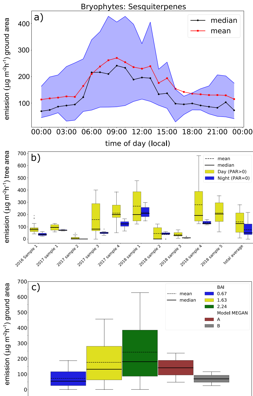
Fig. 2 Sesquiterpene (SQT) emissions from bryophytes of the Amazonian rainforest. a Diel cycle calculated from all 10 bryophyte samples. The blue shaded area extends from the 25th to 75th percentile. b SQT emission boxplots (per tree area) for the 10 different bryophytes samples. The range of emissions during daytime and nighttime is plotted in yellow and blue. The total average boxplots were calculated from all means of the individual samples. c SQT emissions of Amazon bryophytes per ground area for three different bryophyte area indexes (BAI). This is compared to SQT canopy emissions calculated with the MEGAN model (A: Acosta et al., 2014 1 and B: Bourtsoukidis et al., 2018 30 ). The MEGAN boxplots were prepared by using the lower and upper limit for the emissions from the publications, therefore the mean equals the median. The boxes represent the 25th to 75th percentile, the whiskers the 5th to 95th percentile, and both the mean (dashed) and the median values (solid line) are shown.
