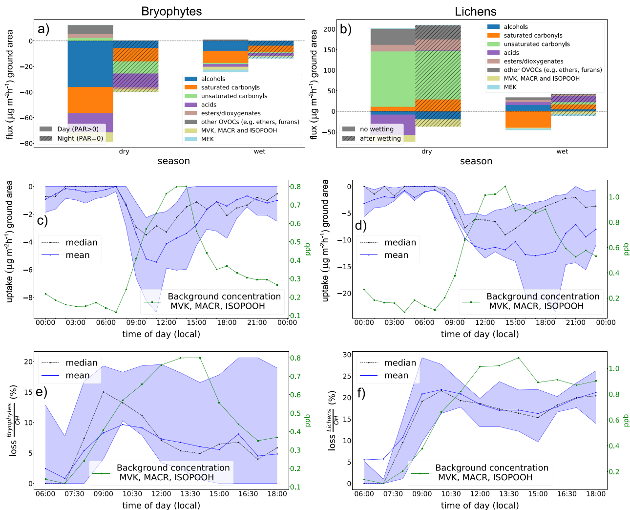
Fig. 5 Emission and uptake of oxygenated volatile organic compounds (OVOCs) and isoprene oxidation products (mass 71: MVK, MACR, ISOPOOH) from bryophytes and lichens of the Amazonian rainforest. Emission and uptake of OVOCs from a bryophytes and b lichens. Diel plots of mass 71 uptake of c bryophytes and d lichens, together with background concentrations of mass 71. Daytime diel plots of the ratio of mass 71 loss via cryptogam uptake to loss by OH oxidation for e bryophytes and f lichens, alongside with the background concentrations of mass 71. Sunrise was around 6:00 local and sunset around 18:00 local. The blue shaded area extends from the 25th to 75th percentile. Diurnal plots were calculated from all bryophyte and lichen samples. The y-axis for the background concentrations (MVK, MACR, ISOPOOH) in the plots c-f is on the right side.
