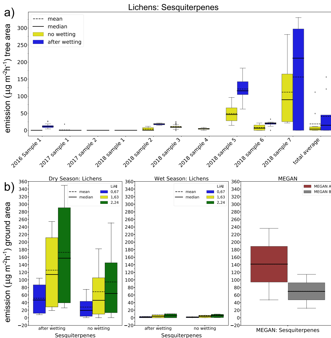
Fig. 4 Sesquiterpene (SQT) emissions from lichen samples of the Amazonian rainforest. a SQT emissions of the 10 individual lichen samples. Emissions before wetting are shown in yellow and after the sample was wetted in blue. The samples 2018 3 and 4 were not wetted. Emissions are shown per tree surface area. The total average boxplots were calculated from all means of the individual samples. b Emissions of SQTs from lichens per ground area. Emission in the dry and wet season for wetted and non-wetted conditions are given for three different lichen area indices (LiAI). The plot on the right is SQT emissions from the canopy calculated with the MEGAN model (A: Acosta et al., 2014 1 and B: Bourtsoukidis et al., 2018 30 ). The MEGAN boxplots were made by using the lower and upper limit for the emissions from the publications, therefore the mean equals the median. The boxes represent the 25th to 75th percentile, the whiskers the 5th to 95th percentile, and both the mean (dashed) and the median values (solid line) are shown.
