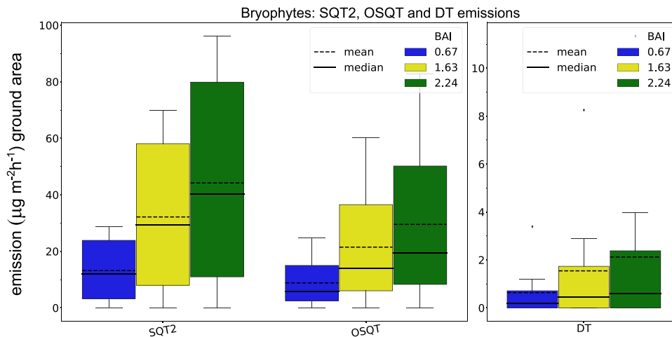
Fig. 3 Bryophytes emissions of SQT2s ( \text{C}_{15}\text{H}_{22} ), OSQTs ( \text{C}_{15}\text{H}_{24}\text{O} ), and DTs ( \text{C}_{20}\text{H}_{32} ). Emissions are per Amazon rainforest ground area for different bryophyte area indices (BAI). The boxes represent the 25th to 75th percentile, the whiskers the 5th to 95th percentile, and both the mean (dashed) and the median values (solid line) are shown.
