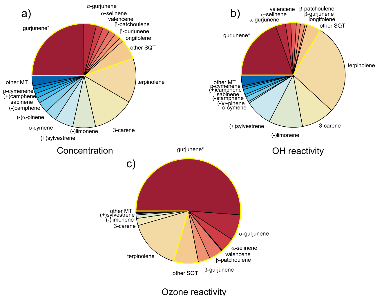
Fig. 6 Contributions of sesquiterpenes and monoterpenes to molar concentration, OH reactivity and ozone reactivity of bryophyte emissions.
