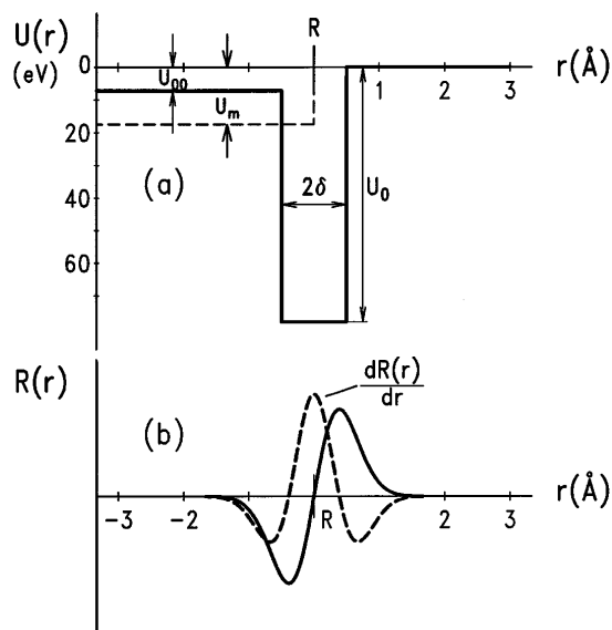
FIG. 2. (a) Simplified potential energy of the final state electron as a function of r for cases A and B (dotted and solid lines). (b) Schematic representation of the symmetry of radial wave function R_i(r) of the initial HOMO and HOMO-1 states along with its derivative.
