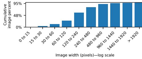
Fig. 8. Cumulative distribution of image widths on the landing pages of the Alexa top 500 websites. Over 80% of the images have widths under 480 pixels. Narrower images have a higher transition rate, and thus higher relative overheads when using expensive transitions.
