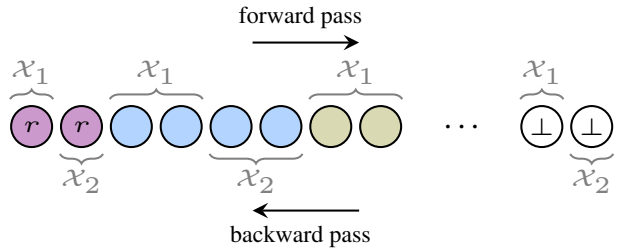
Figure 4. Arrangement of BDD nodes in GPU memory for the ILP in Figure 2. For the forward pass in Alg. 1 we proceed from root to terminal nodes and vice versa for the backward pass.
