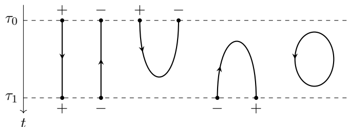
Figure 5. All possible connected oriented bordisms. We call them positively and negatively oriented intervals, left elbow, right elbow, and circle, respectively. The cut functions are \rho_i = t - \tau_i , so these pictures are read from top to bottom.
