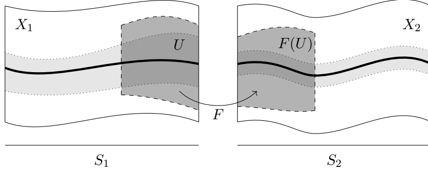
Figure 3. Picture of an object in \mathcal{GBord}_0(\{S_1, S_2 \rightarrow S\}) . The light shaded regions depict the neighborhoods (\rho_0^i)^{-1}(-\varepsilon, \varepsilon) of the core (X_i)_0^0 (drawn as a thick line). When attempting to glue, the difficulty is to shrink X_i to \tilde{X}_i in such a way that the corresponding restriction \tilde{F} of F maps \tilde{X}_1|_{S_{12}} diffeomorphically to \tilde{X}_2|_{S_{12}} .
