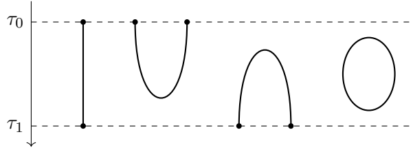
Figure 4. All possible connected unoriented one-dimensional bordisms. We call them interval, left elbow, right elbow, and circle, respectively. The cut functions are \rho_i = t - \tau_i , so these pictures are read from top to bottom.
