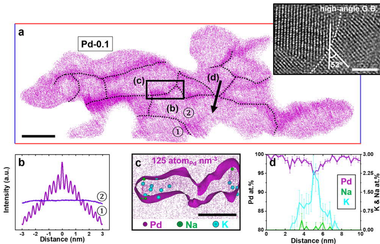
Figure 2. Grain boundary studies for Pd-0.1 nanogels. (a) A 1 nm thin-sliced tomogram from a 3D atom map (Figure S5) of Pd-0.1 gels (isocomposition surface >90 at. % Pd). The scale bar is 10 nm. The dotted black line represents grain boundary features. The inset shows a high-resolution TEM image of Pd-0.1 (scale bar is 2 nm). (b) Spatial distribution maps along the z -axis from the grains of two different nanogels. (c) Extracted grain boundary tomogram with the isodensity surface of 125 Pd atoms/nm 3 . The scale bar is 5 nm. (d) 1D compositional profiles of detected Na, K, and Pd elements.
