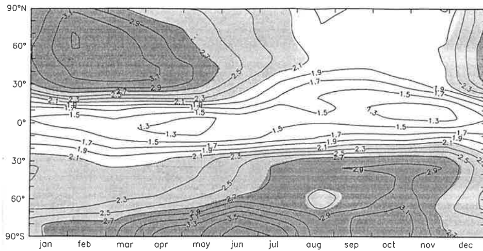
Zonal mean Be-10/Be-7 concentration ratio (11. model level)
