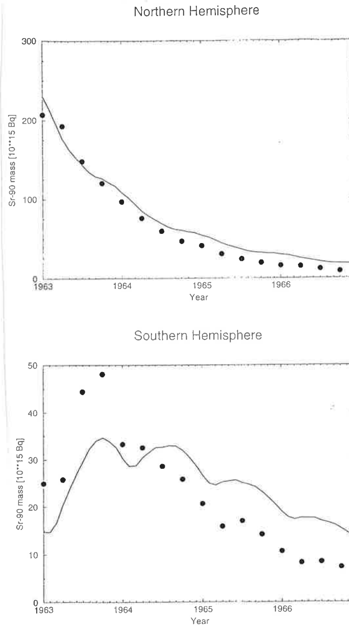
Fig.14 Time development of northern stratospheric (upper panel) and southern stratospheric (lower panel) 90 Sr mass [10 15 Bq] during the 4-year simulation period from 1963 till 1966. The solid line represents the model, the points denote observations compiled by Staley (1982).
