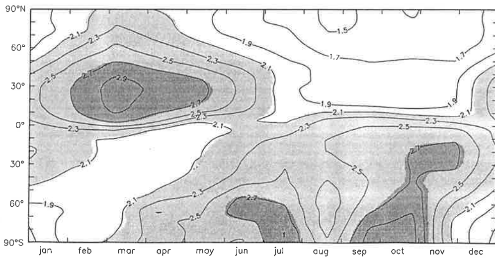
Zonal mean Be-10/Be-7 concentration ratio (lowest model level)
