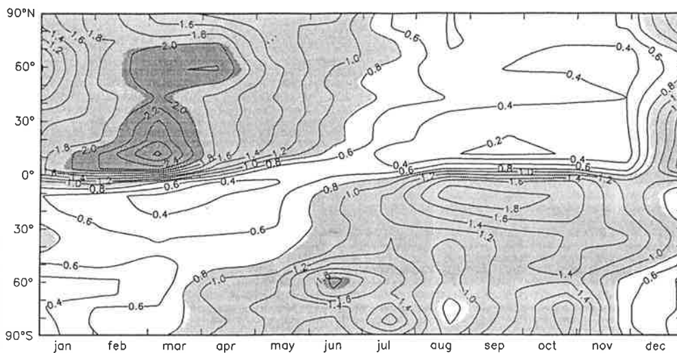
Monthly mean Sr-90 concentration / yearly mean Sr-90 concentration (lowest model level)
