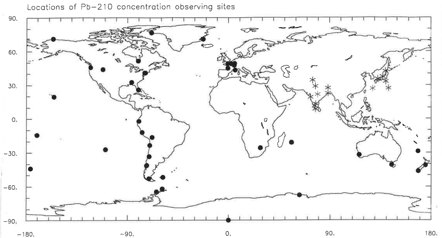
Fig.1 Monthly station observations of ^{210}\text{Pb} concentration. Solid circles mark stations with measurements from 1990, stars denote sites with observations from other years (see text).
