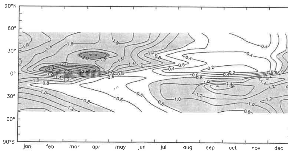
Monthly mean Sr-90 concentration / yearly mean Sr-90 concentration (Observations)
