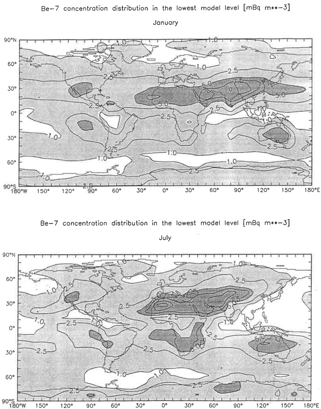
Fig.9 7 Be concentration distribution [mBq m -3 ] in the lowest model level for January (upper panel) and July (lower panel).
