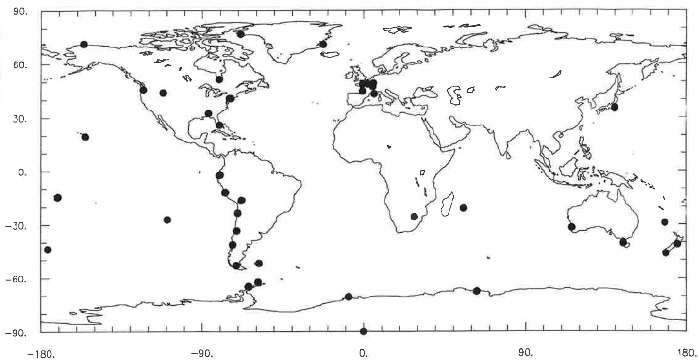
Locations of Be-7 concentration observing sites
