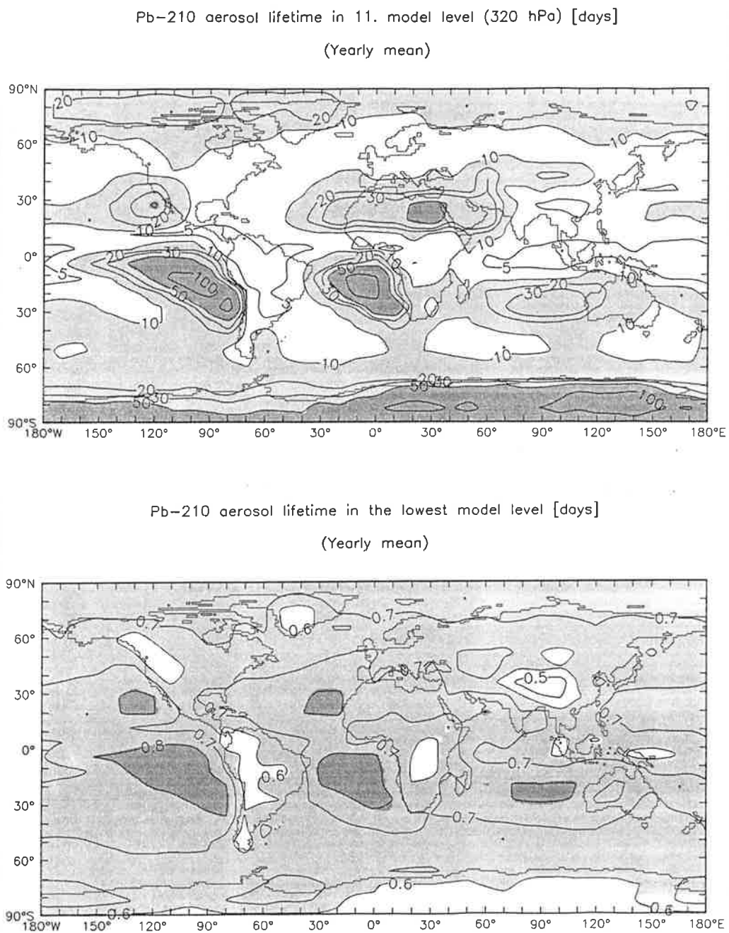
Fig.4 Yearly mean of ^{210}\text{Pb} aerosol lifetime [days] in the lowest (lower panel) and 11. model level (320 hPa, upper panel).
