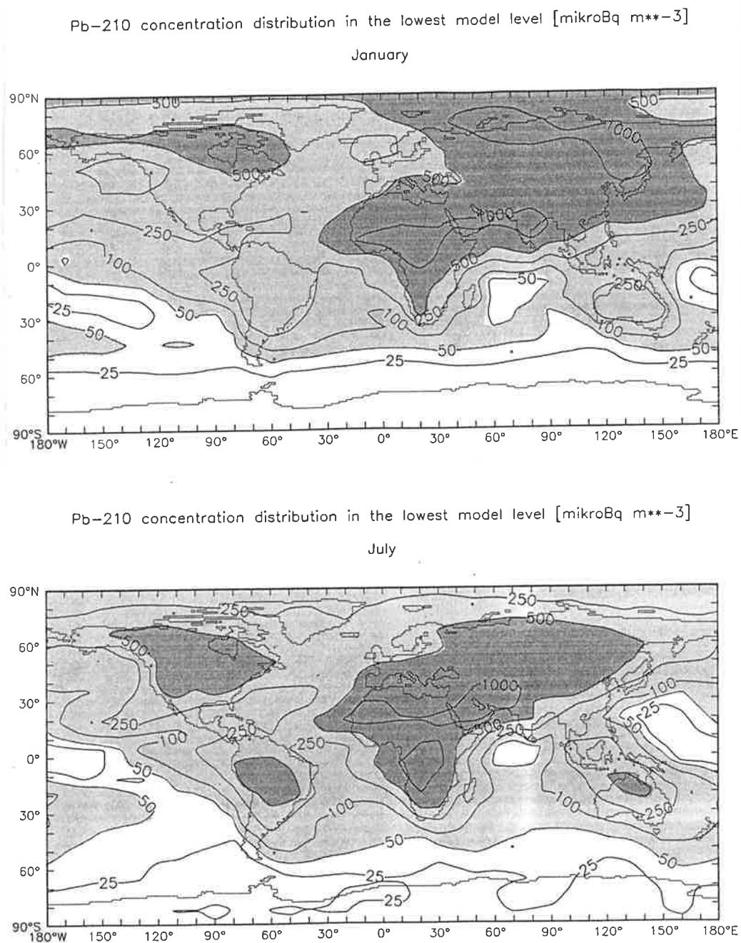
Fig.7 210 Pb concentration distribution [ \mu\text{Bq m}^{-3} ] in the lowest model level in January (upper panel) and July (lower panel).
