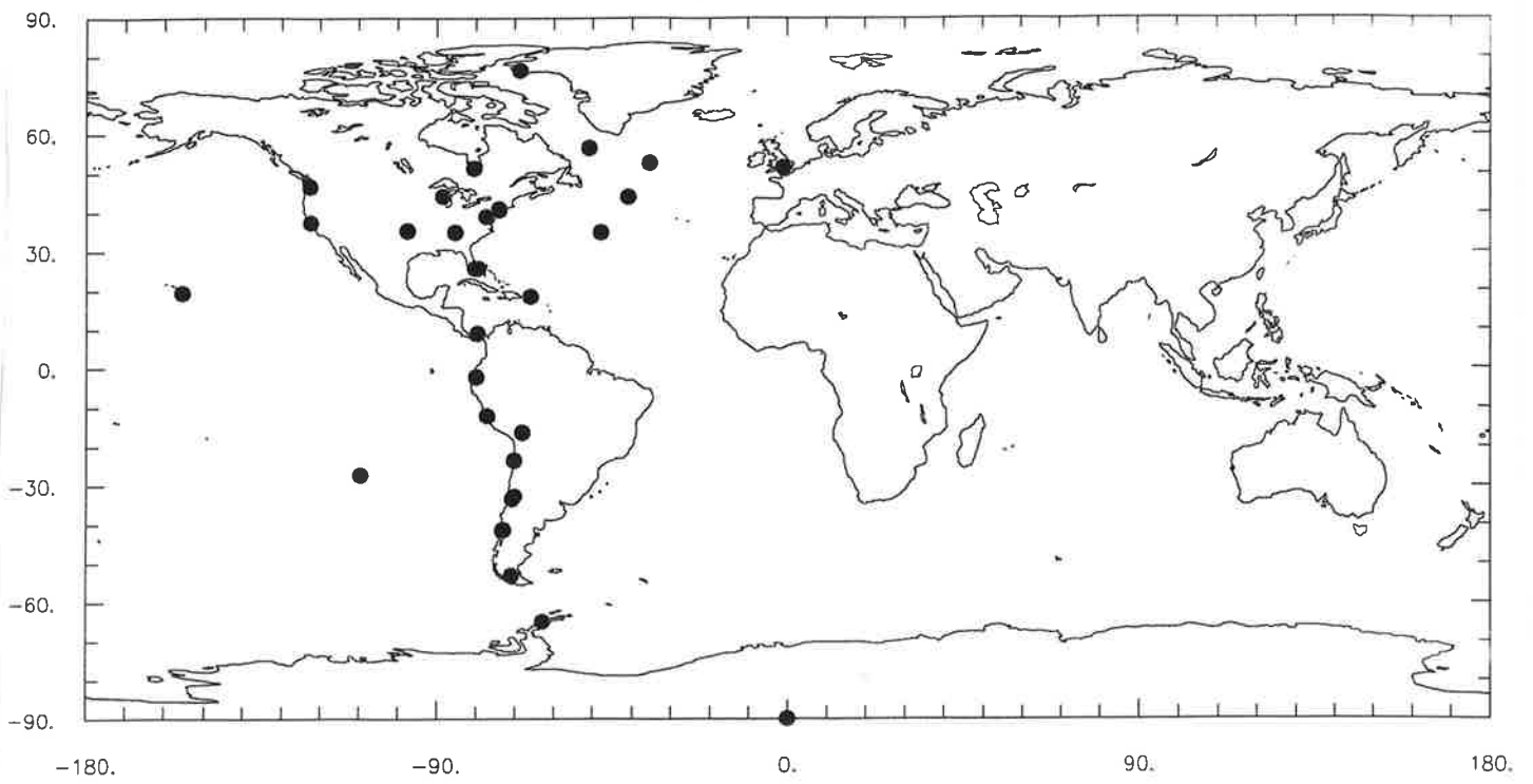
Locations of Sr-90 concentration observing sites
