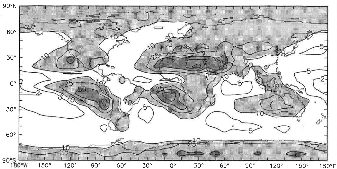
Percentage of dry Pb-210 deposition with respect to total Pb-210 deposition (Yearly sum)
