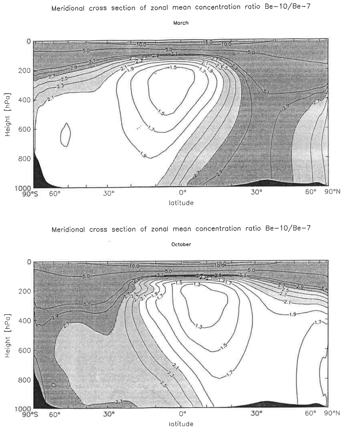
Fig.10 Meridional cross section of modelled zonal mean concentration ratio ^{10}\text{Be}/^{7}\text{Be} for March (upper panel) and October (lower panel).
