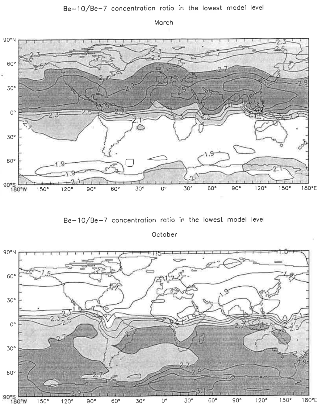
Fig.11 Concentration ratio ^{10}\text{Be}/^{7}\text{Be} in the lowest model level for March (upper panel) and October (lower panel).
