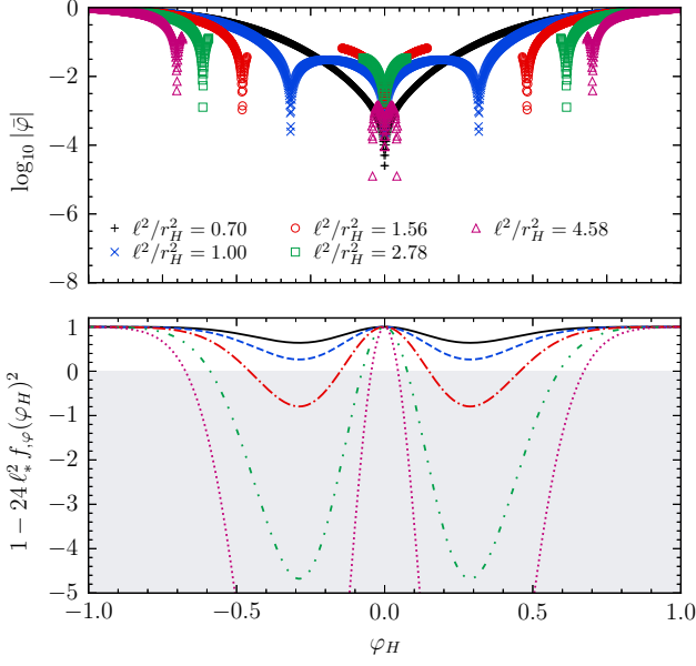
FIG. 12. Finding scalarized black hole solutions in the Gaussian theory (42). Top panel: the asymptotic value \log_{10} |\bar{\varphi}| of the scalar field as a function of its value at the horizon \varphi_H for several ratios \ell_* = \ell/r_H . When \ell_*^2 \lesssim 0.725 only one zero of \bar{\varphi} , located at \varphi_H = 0 exists as shown by the cusps in the data points. It corresponds to the Schwarzschild solution. As we increase \ell_* , two additional zeros of \bar{\varphi} with \varphi_H \neq 0 appear. They have the same magnitude, but opposite signs, as expected from the theory’s \mathbb{Z}_2 -symmetry. Note that for \ell_*^2 = 1.56, 2.78 and 4.58 the curve is not continuous. Bottom panel: the existence condition (12) as a function of \varphi_H . The solid, dashed, dot-dashed, dash-double-dotted and dotted lines correspond respectively to \ell_*^2 = \{0.7, 1.0, 1.56, 2.78, 4.58\} . In the shaded region, Eq. (12) is violated. For \ell_*^2 = 1.56 and 4.58 , the condition is violated on \varphi_H intervals. This causes the discontinuity in the data points with the same values of \ell_* in the top panel.
