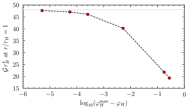
FIG. 3. Numerical Gauss-Bonnet scalar \mathcal{G} r_H^4 evaluated at the event horizon r_* = r/r_H = 1 for a sequence of black holes with constant (\ell/\mu)^2 = 10^{-1} . As the scalar field at the horizon \varphi_H approaches its maximum allowed value \varphi_H^{\max} \approx 3.77526 , the Gauss-Bonnet scalar tends to the limit \mathcal{G} r_H^4 = 48 (horizontal line) predicted analytically by Eq. (18a).
