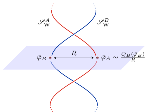
FIG. 7. Illustration of the two-body dynamics. Two black holes with ADM masses and scalar charges M_A(\bar{\varphi}_A) , Q_A(\bar{\varphi}_A) = -M_A(\bar{\varphi}_A)\alpha_A(\bar{\varphi}_A) and their B counterparts are inspiralling at fixed irreducible masses \mu_A and \mu_B . In the previous sections, we calculated these quantities non perturbatively. The background scalar field \bar{\varphi}_A , experienced by black hole A , can now be estimated at leading-order by the \propto 1/R potential (48a) sourced by black hole B , and vice-versa. The values of \bar{\varphi}_A and \bar{\varphi}_B change as the orbital radius R decreases.
