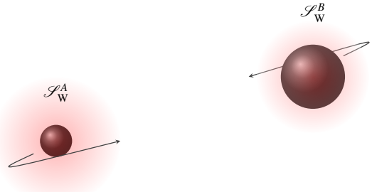
FIG. 1. Illustration of the problem. Two black holes with Arnowitt-Misner-Deser (ADM) masses M_{A,B} and with scalar charges Q_{A,B} are in a binary system. The scalar field of each black hole affects its companion, altering its mass and scalar charge. In the PN regime, and when finite-size corrections (e.g. tidal and out-of-equilibrium effects) can be neglected, these changes take place adiabatically, keeping the Wald entropy \mathcal{S}_W^{A,B} of each black hole constant. The change in the mass due to a slowly-varying scalar field environment at constant Wald entropy is the sensitivity, which we calculate here.
