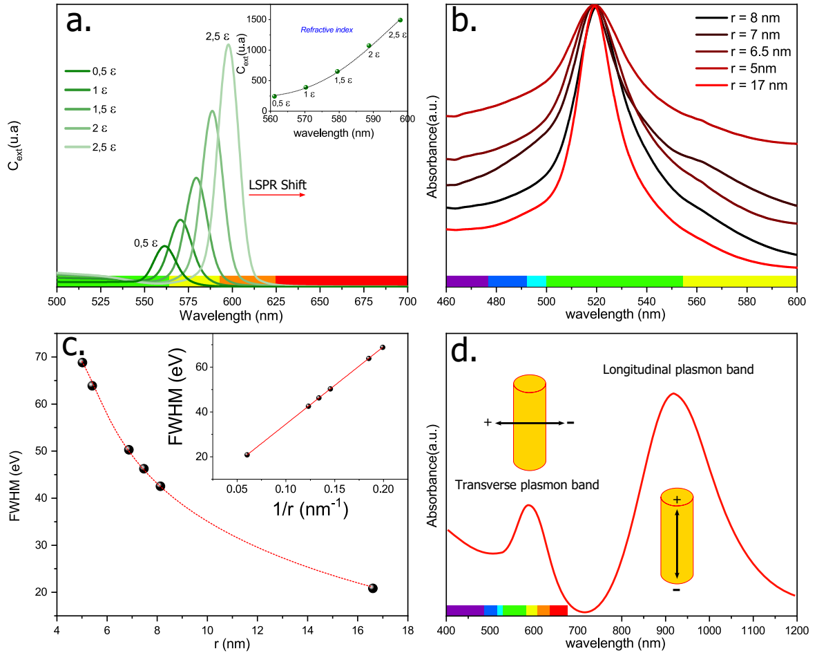
Figure 3.3: (a.) LSPR shift of colloidal gold nanoparticles in different refractive indexes \epsilon . (b.) Change in the Full Width at Half Maximum (FWHM) of the absorption band due to the change of particle size. (c.) inverse relation of FWHM and particle size r . (d.) Creation of two absorption bands in optical spectra of gold nanorods due to the influence of shape over the LSPR.
