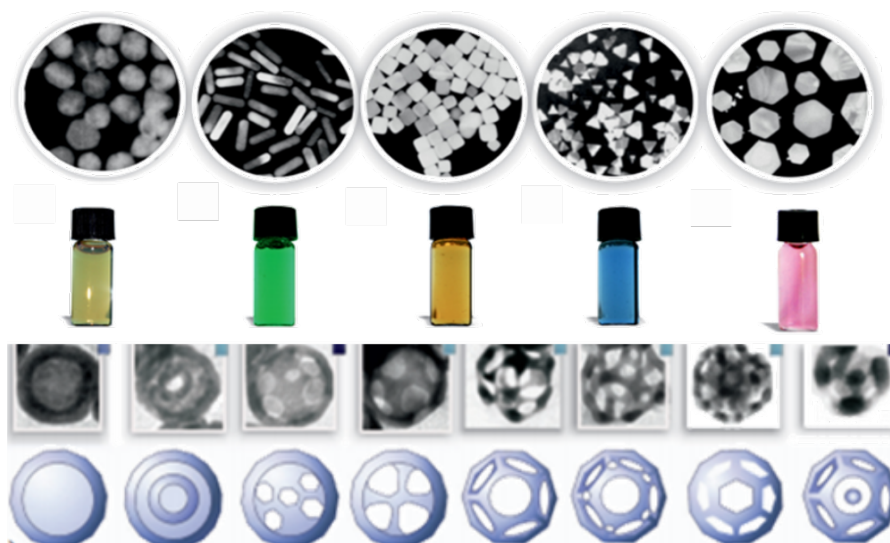
Figure 1.3: Shape variation in a collection of colloidal AuNPs as a function of color. The lower part shows the topological condition obtained by the scaling law. Figure extracted from Edgar González et. al.-2011 [1] and [2]
