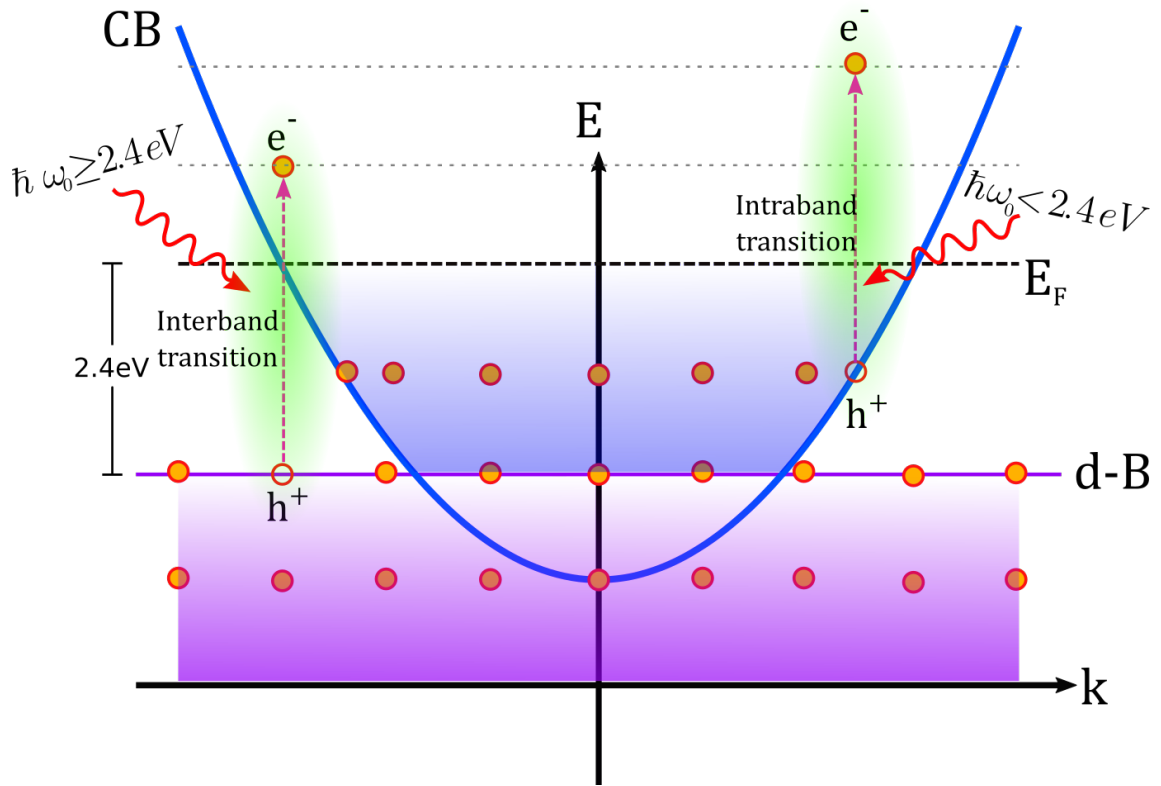
Figure 3.9: Schematic representation of plasmon decay process. Radiative by emitting a photon or Non-radiative by generating electron-hole pairs
