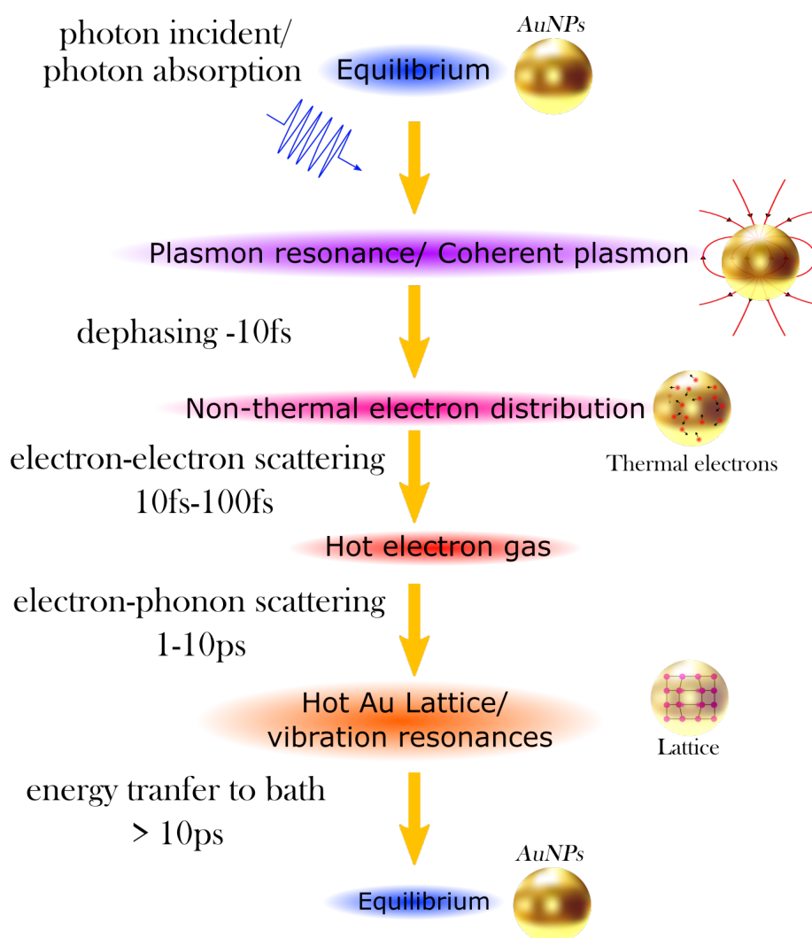
Figure 6.6: Diagram of lifetime plasmon. A sequence of lifetime plasmon and approximate time scales.
