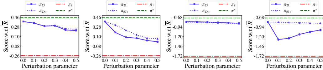
(a) Navigation, PreAttack (b) Navigation, PostAttack (c) Grid world, PreAttack (d) Grid world, PostAttack
