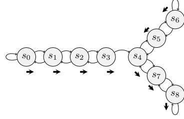
(a) The navigation environment
