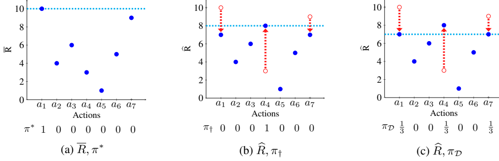
Figure 5: A single-state environment with 7 actions. In each figure, the denoted policy is uniform over actions on or above the dashed line. (a) shows \bar{R} and \pi^* . Here, the optimal policy selects action a_1 . (b) shows \hat{R} and target policy \pi_{\dagger} with \epsilon_{\dagger} = 1 . Here, the target policy selects action a_4 . (c) shows \hat{R} and \pi_{\mathcal{D}} with \epsilon_{\mathcal{D}} = 2 . The defense strategy only sees poisoned rewards \hat{R} , so it first calculates the optimal action and the set of all second best actions under \hat{R} , in this case \{a_1, a_7\} , which then form the set \Theta_s^\epsilon = \{a_1, a_7\} . To obtain defense policy \pi_{\mathcal{D}} , we can solve the optimization problem (P3b), which implies that \pi_{\mathcal{D}} should select an action uniformly at random from the set \{\pi_{\dagger}(s)\} \cup \Theta_s^\epsilon = \{a_1, a_4, a_7\} .
