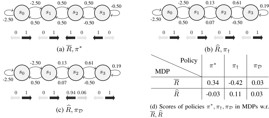
Figure 1: A simple chain environment with 4 states and two possible actions: left and right . s_0 is the initial state. The agent goes in the direction of its action with probability 90%, and otherwise the next state is selected uniformly at random from the other 3 states. Weights on edges indicate rewards for the action taken. For example in Fig. 1a, if the agent takes left in state s_1 , it receives 0.5. We denote the true rewards by \bar{R} , the poisoned rewards by \hat{R} , the optimal policy under \bar{R} by \pi^* , the target policy (which is uniquely optimal under \hat{R} ) by \pi_{\dagger} , and the defense policy (which is derived from our framework) by \pi_{\mathcal{D}} . (a) shows \bar{R} and \pi^* . In particular, the numbers above the arrows and the different shades of gray show the probabilities of taking actions left and right under \pi^* . (b) shows \hat{R} and \pi_{\dagger} . (c) shows \pi_{\mathcal{D}} that our optimization framework derived from \hat{R} , and by reasoning about the goal of the attack ( \pi_{\dagger} ). In particular, our optimization framework maximizes the worst-case performance under \bar{R} : while the optimization procedure does not know \bar{R} , it can constrain the set of plausible candidates for \bar{R} using \hat{R} . (d) Table. 1d): Each entry in the table indicates the score of a (policy, reward function) pair, where the score is a scaled version of the total discounted return (see Section 3). For example, the score of policy \pi_{\dagger} equals -0.42 and 0.11 under \hat{R} and \bar{R} respectively. Our defense policy significantly improves upon this and achieves a score of 0.03 . For comparison, the score of \pi^* equals 0.34 . Moreover, unlike for the target policy \pi_{\dagger} , the score of our defense policy \pi_{\mathcal{D}} under \bar{R} is always at least as high as its score under \hat{R} , as predicted by our results (see Theorem 1). The results are obtained with parameters \epsilon_{\dagger} = 0.1 , \epsilon_{\mathcal{D}} = 0.2 and \gamma = 0.99 (see Section 3).
