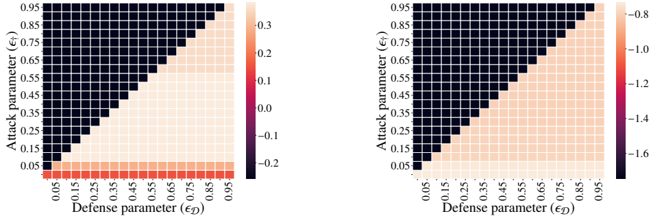
(a) \bar{\rho}^{\pi_D} in the navigation environment. For comparison, \bar{\rho}^{\pi_{\dagger}} = -0.26 and \bar{\rho}^{\pi^*} = 0.45 .
