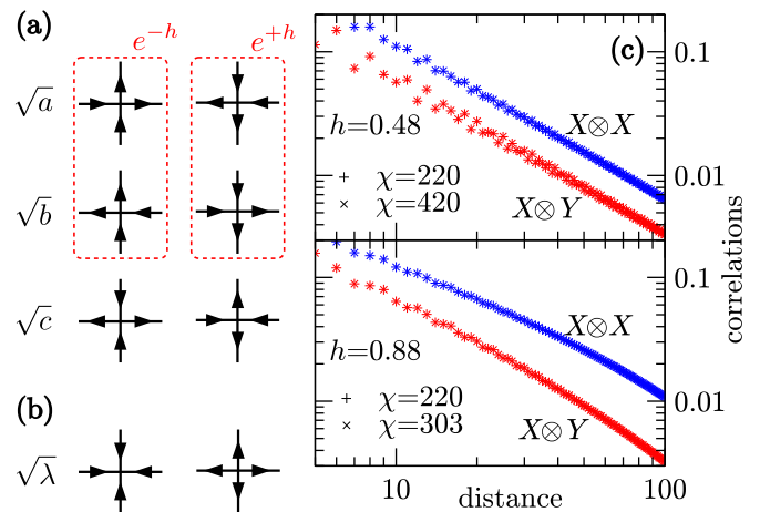
FIG. 4. PEPS with emergent U(1) symmetry. (a) 6-vertex model with magnetic field h ; we choose a = b = 1 , c = 3 . The corresponding PEPS (the superposition of all 6-vertex configurations with the indicated amplitude) has K < \frac{1}{2} for suitable h . (b) Perturbation breaking the U(1) symmetry. (c) Decay of correlations related by U(1) but not \mathbb{Z}_2 symmetry. The identical decay scaling at h = 0.48 ( K = 0.435 ) is consistent with an emergent U(1) symmetry in the correlations, while the different decay at h = 0.88 ( K = 0.593 ) rules it out. The data is converged in the CTM bond dimension \chi .
