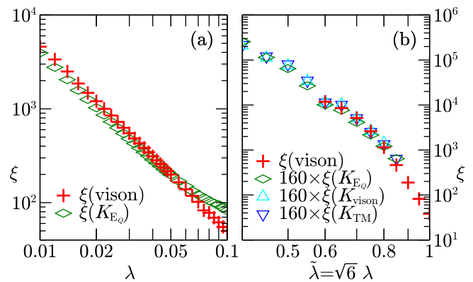
FIG. 3. Correlation length \xi(\text{vison}) in the vison sector, and fits \xi(K) obtained from the sine-Gordon model. (a) Dimer-solidomer interpolation. (b) RVB model with LR-singlets, using the K of Fig. 2.
