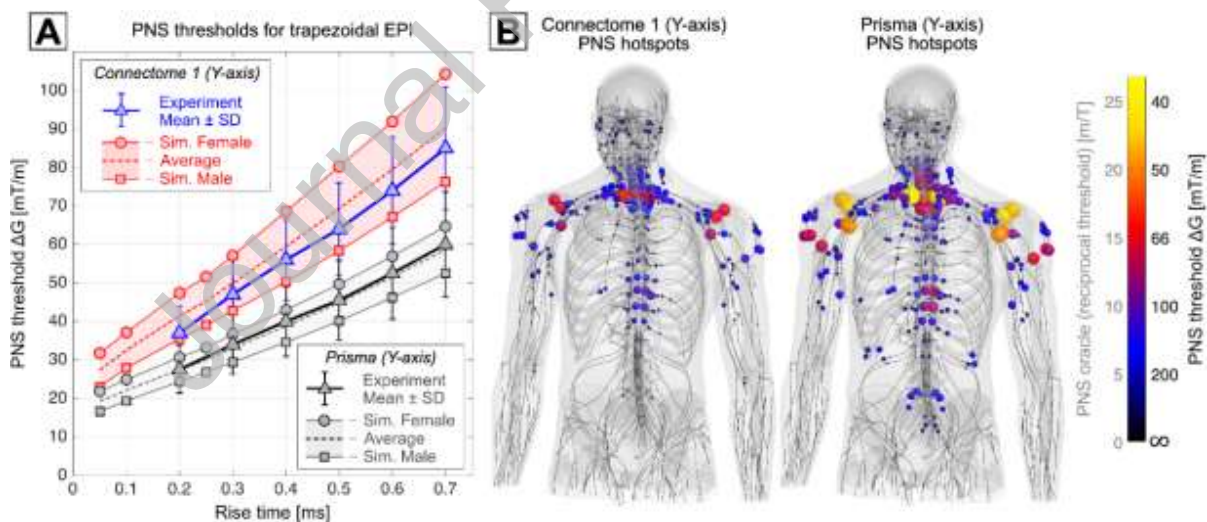
Figure 4. Peripheral Nerve Stimulation (PNS) Simulations. A: Experimental and simulated PNS threshold curves given as minimum stimulating gradient amplitude \Delta G as a function of rise time for the y-axis of the Connectome gradient (experiments in blue, simulation in red) and the Prisma gradient (in grayscale). PNS thresholds were obtained for a trapezoidal bipolar train with 0.5 ms flat top duration. B: Simulated activation maps plotted as PNS oracle hot-spots
