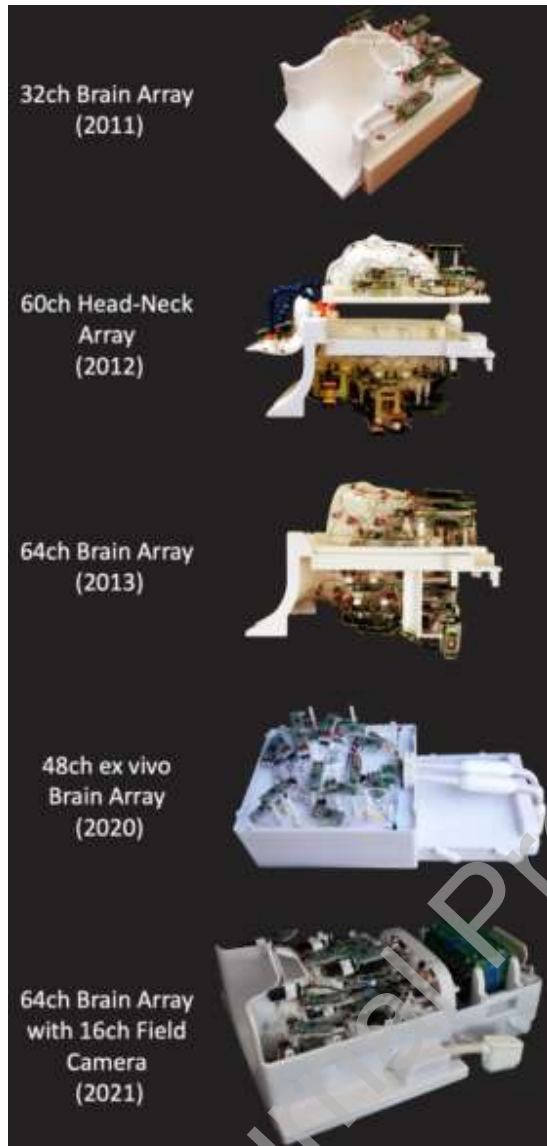
Figure 5. Select array coils developed for the Connectome MRI scanner. Starting in 2011 with a 32-channel head coil, Connectome coil technology has evolved from a 60-channel head-neck array, a 64-channel brain array, and a 48-channel ex vivo brain coil all the way to a 64-channel head coil with an integrated field monitoring system in 2021. Figure adapted from (Keil et al., 2013; Mahmutovic et al., 2021; Scholz et al., 2021)
