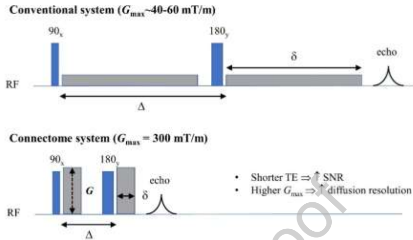
Figure 1. Benefits of strong gradients for diffusion MRI. Higher gradient amplitudes up to 300 mT/m on the Connectome system (bottom) achieve a given diffusion-encoding gradient area in less time compared to conventional gradient systems (top), as illustrated through the pulsed gradient spin echo diffusion MRI sequence. Benefits of strong diffusion-encoding gradients include shortening the entire diffusion-encoding period and echo time (TE), and hence increasing the signal-to-noise ratio (SNR) by reducing signal loss due to T2 decay. The larger gradient amplitudes also enable stronger diffusion encoding (i.e., larger diffusion-encoding gradient areas, larger q -values and b -values) to be achieved with shorter diffusion times, providing higher “diffusion resolution” to improve the capability of resolving smaller length-scales for probing tissue microstructure and for resolving complex white matter structures such as crossing fibers. RF = radiofrequency, \delta = diffusion-encoding gradient pulse duration, \Delta = diffusion time.
