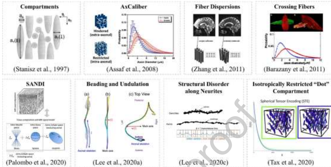
Figure 12. Illustration of diffusion models and key concepts. The concept of compartmentalization was initially proposed by Stanisz et al. (a), following which the AxCaliber aims to estimate the diameter distribution of the restricted water compartment (b). Variations of the AxCaliber model was proposed, such as modifications to account for fiber dispersions (c) and crossings (d). Realistic axons are very different from ideal cylinders, instead, there are plenty of beadings and undulations (f) and structural disorder are commonly seen along neurites (g). In gray matter, a sphere (e) or dot (h) compartment is incorporated into the physical model to account for additional signal component present in the measurement. Figure adapted from the papers labeled therein.
