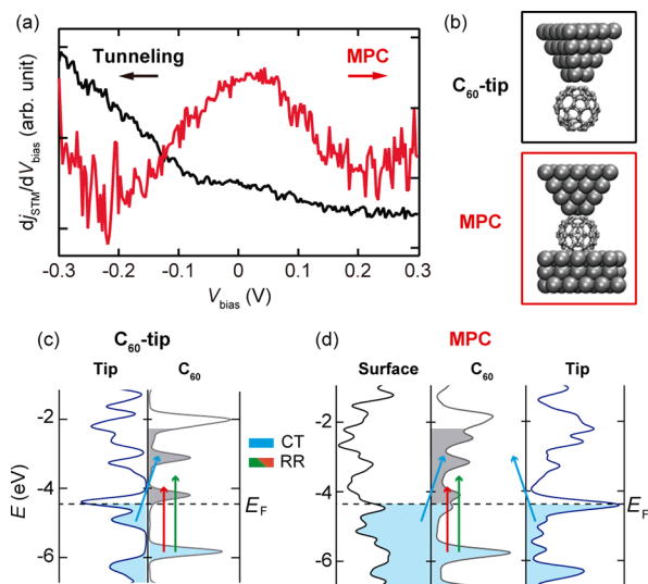
Figure 5. (a) Scanning tunneling spectra obtained for a C_{60} -tip in the tunneling and MPC (black: set-point of V_{bias} = -300 mV, j_{STM} = 5 nA, V_{mod} = 5 mV at 883 Hz, red: set-point of V_{bias} = -300 mV, j_{STM} = 27 \mu A, V_{mod} = 5 mV at 883 Hz). (b) Models of C_{60} -tip and MPC used in the DFT calculations. (c,d) Calculated projected density of states for C_{60} -tip and MPC. The arrows show possible resonance paths in the system (blue arrow: CT, red/green arrows: molecular resonance). The gray areas represent the molecular unoccupied states that can be reached with \lambda_{ext} = 532 nm.
