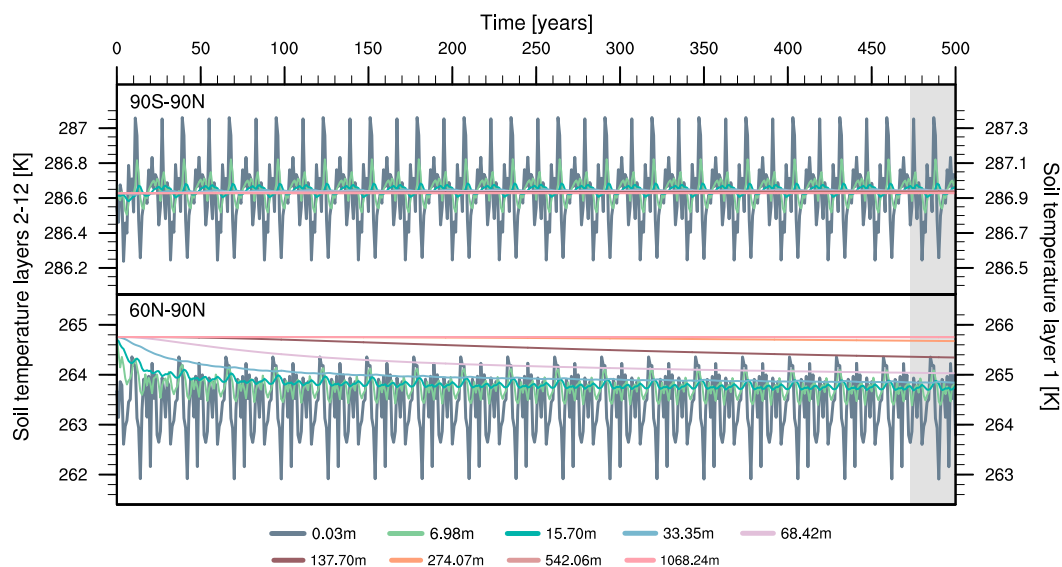
FIG. 3. (top) Global and (bottom) Northern Hemisphere high-latitude ( 60^{\circ} – 90^{\circ} N) subsurface temperature (K) in the 12L deep land surface model configuration in the PIC simulation of 500 years. The uppermost subsurface layer (solid gray) corresponds to the temperature scale on the right, all other layers correspond to the temperature scale on the left. The gray shaded area (years 473–500) corresponds to the last 28-yr chunk of the driving boundary conditions (see text for details). Layers 2–4 are not included to enhance visibility.
