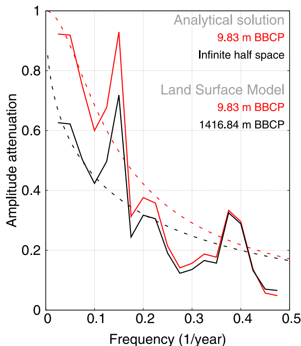
FIG. 4. Ratio of spectral amplitude estimates for the temperature time series at the first and fifth model layers using the shallow 5L (solid red) and 12L deep model (solid black) for a grid point at 27.0°N, 5.6°E. Spectral estimates have been obtained from the last 100 years in the piControl simulations using Welch’s periodogram (Stoica and Moses 1997). Dashed lines correspond to analytical estimates of the conductive attenuation expected at each frequency for a 9.83 m shallow and an infinite half space (Smerdon and Stieglitz 2006).
