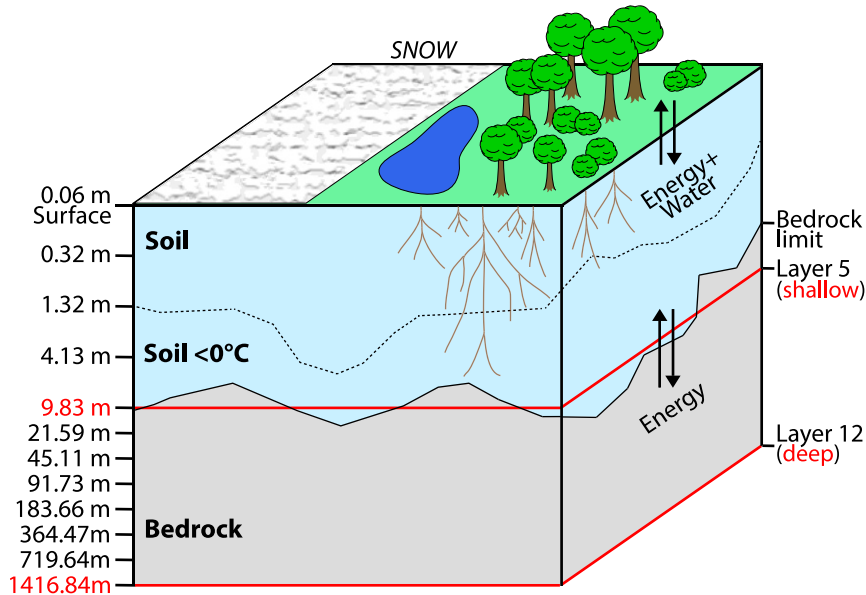
FIG. 1. Vertical structure of the JSBACH LSM version used herein. The scheme corresponds to an example of grid points with frozen soil and partial snow cover, e.g., in northern high latitudes; see also Part II for comparison. The numbers left of the soil column show the depths of the bottom of each layer. Red lines indicate the downward expansion of the BBCP with seven more layers.
