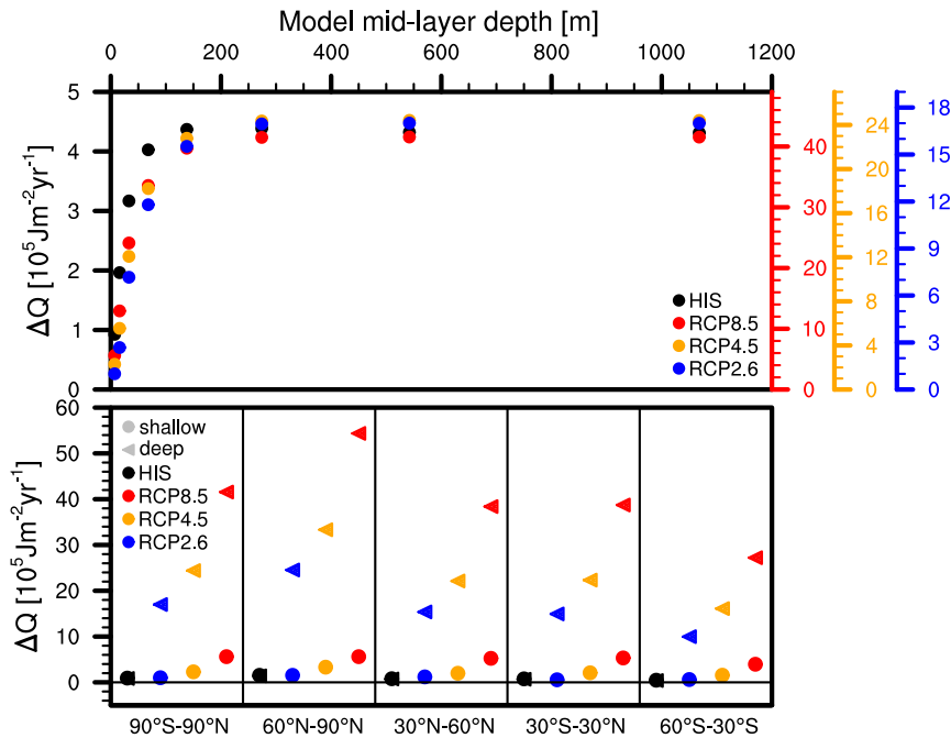
FIG. 12. (top) Global mean annual heat content change ( 10^5 \text{ J m}^{-2} \text{ yr}^{-1} ) in dependence to BBCP-depth configuration for HIS (left axis) and the RCP simulations (right axis). Results are shown for stepwise increases from the 5 to the 12L configuration. (bottom) Area mean annual heat content change ( 10^5 \text{ J m}^{-2} \text{ yr}^{-1} ) in the shallow (circles) and deep (triangles) LSM configurations, for global, NH high latitudes, NH midlatitudes, intertropical regions, SH midlatitudes, and SH high latitudes.
