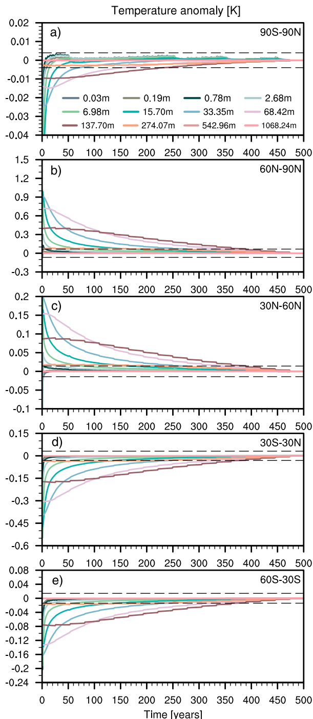
FIG. 5. Soil temperature anomalies (K) in the 12L PIC experiment with respect to the last 28 years (years 473–500 in the shaded time interval in Fig. 3) of the simulation for (a) global (90°S–90°N), (b) Northern Hemisphere high latitudes (60°–90°N), (c) Northern Hemisphere midlatitudes (30°–60°N), (d) low latitudes (30°S–30°N), and (e) Southern Hemisphere midlatitudes (60°–30°S). Dashed lines depict two standard deviations from the mean for the resulting anomalies in the 500 years of simulation. Note the differences in the temperature y-axis scales.
