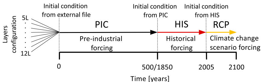
FIG. 2. Experimental setup for the JSBACH simulations with gradually increasing layer configurations from 5 to 12 layers (5L–12L) under preindustrial, historical, and twenty-first-century climate change (RCP) forcing scenarios. The preindustrial control simulation (PIC) is performed for 500 years with conditions of 1850 to reach temperature equilibrium in the subsurface layers, before running the consecutive historical (HIS) and future scenario (RCP) simulations.
