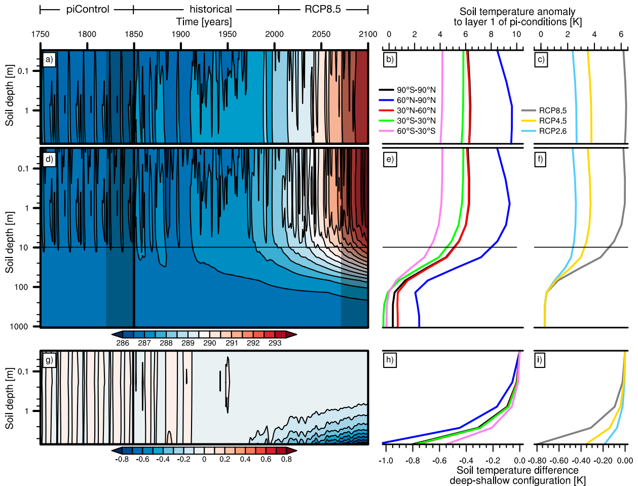
FIG. 7. Hovmöller diagram of the absolute global temperature (K) vs depth (m) for the last 100 years in the piControl simulation (dates are arbitrary and do not correspond to actual dates in forcing in PIC) continued into the historical (1850–2005) and RCP8.5 (2006–2100) simulations for (a) the 5L configuration, (d) the 12L configuration, and (g) soil temperature differences (K) for the first 5 layers in between the deep 12L and the shallow 5L configurations. Soil temperature anomaly profiles for the last 30 years in the RCPs scenario ( \bar{T}_{2071-2100} ; dark shaded area) relative to the temperatures of the first soil level at the end of the piControl simulation ( \bar{T}_{1825-1850} ; dark shaded area) for the (c) shallow 5L and (f) deep 12L configurations and (i) the differences between them for the first 5 model layers. For the RCP8.5, profiles are shown specifically also for several latitudinal bands for the (b) shallow, (e) deep, and (h) differences.
