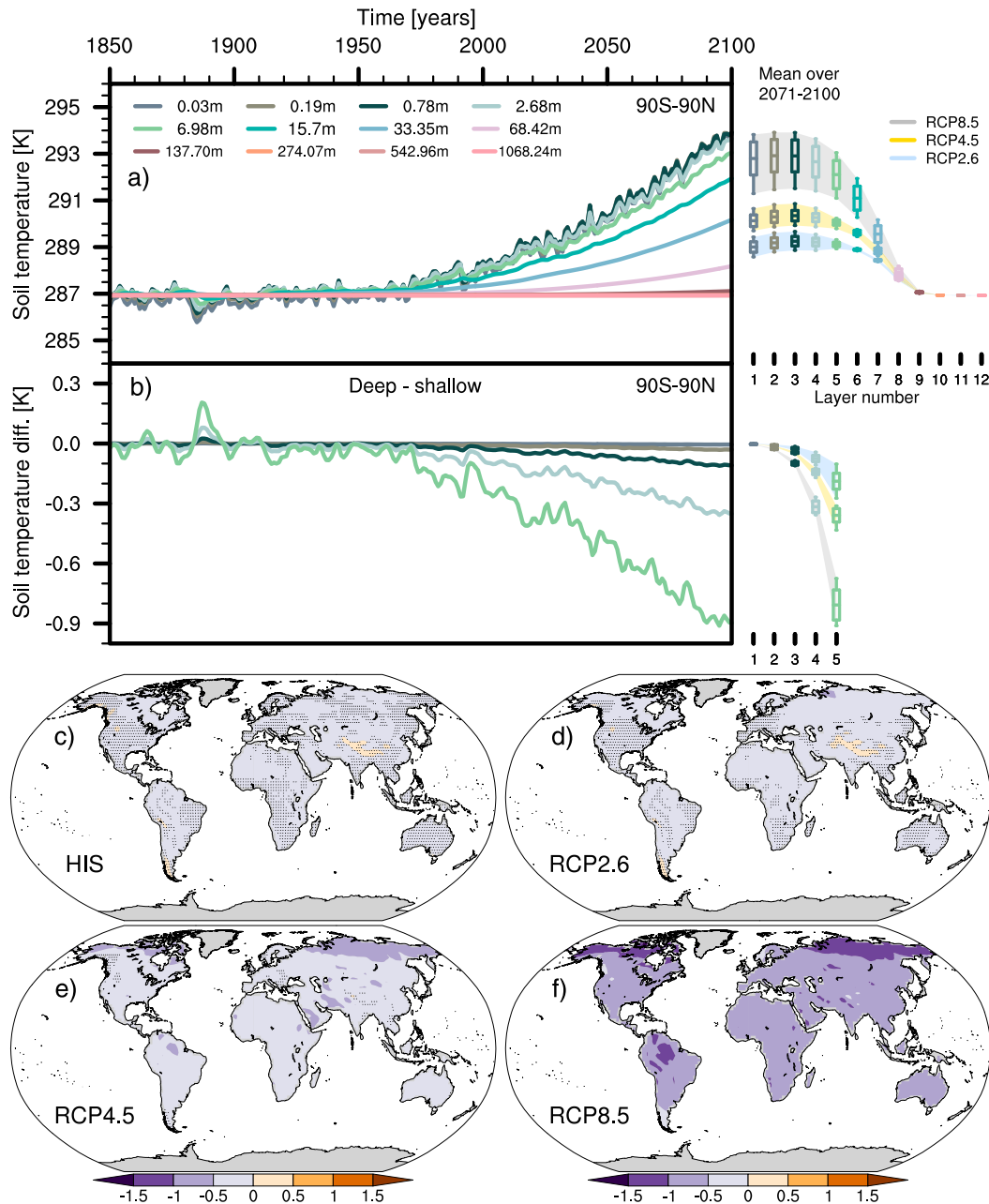
FIG. 6. (a) Global absolute soil temperatures (K) in the 12L LSM configuration and (b) differences between the 12L and 5L configurations for the top 5 LSM layers in the historical and RCP8.5 simulations. Box-and-whisker plots indicate the (a) range of temperature variability and (b) differences for each soil layer and in the three RCP scenarios during the last 30 years of simulation. Box length stands for a range of two standard deviations, with the mean mark inside and the whiskers showing the levels for the minimum and the maximum. (c)–(f) Soil temperature differences (K) between the deep 12L and the shallow 5L configuration at the fifth layer (9.83 m) of the last 30 years of the historical (HIS) simulation, the RCP2.6, RCP4.5, and RCP8.5 simulations. Points without stippling show significant differences (Student’s t test, p < 0.05 ).
