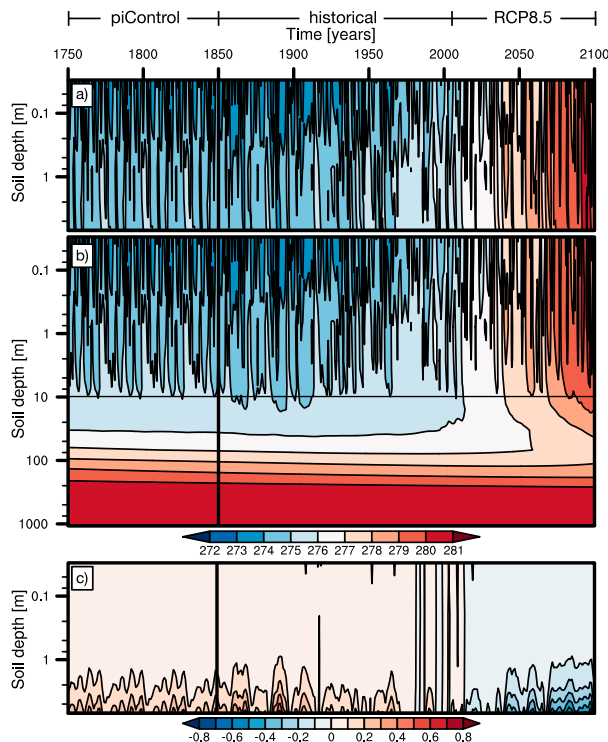
FIG. 11. Hovmöller diagram of the absolute temperatures (K) vs depth (m) at a grid point in the western United States ( 45.7^\circ\text{N} , 112.5^\circ\text{W} ) for the last 100 years in the piControl simulation (dates are arbitrary and do not correspond to actual dates in forcing in PIC) continued into the historical (1850–2005) and RCP8.5 (2006–2100) simulations for (a) the 5L configuration, (b) the 12L configuration, and (c) soil temperature differences (K) for the first 5 layers in between the deep 12L and the shallow 5L configurations.
