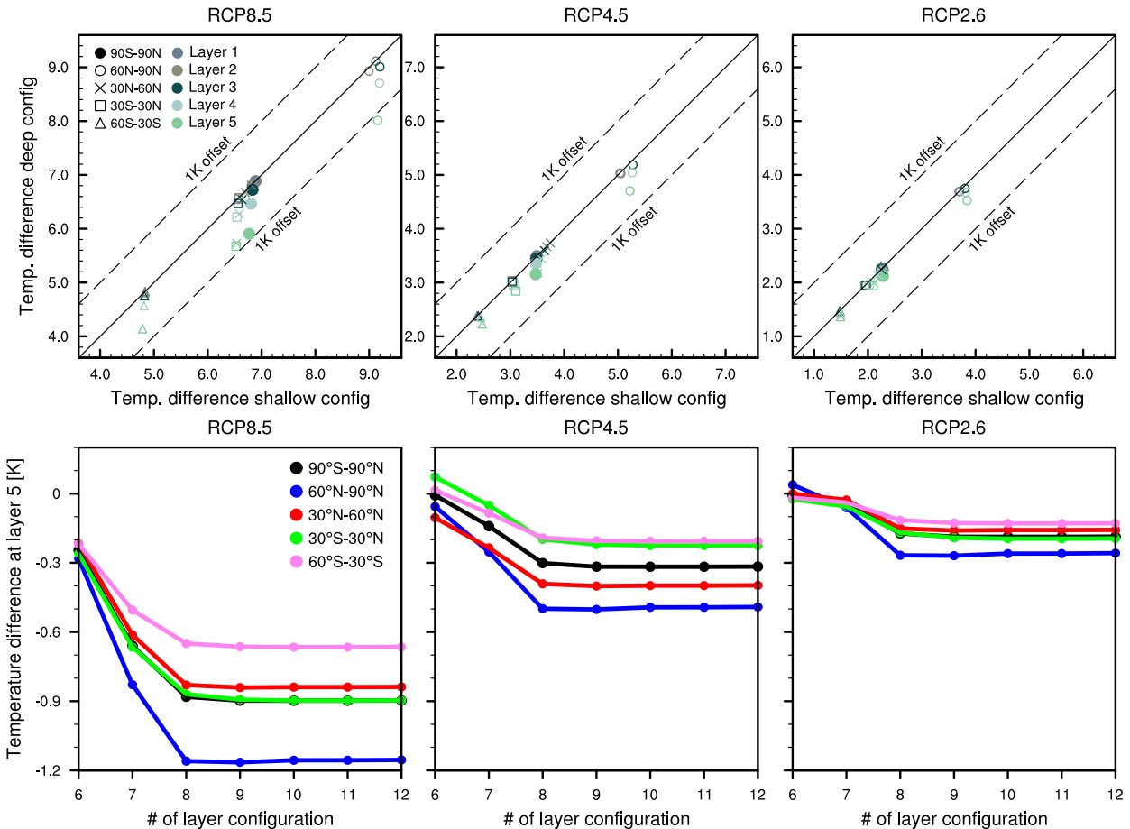
FIG. 9. (top) Subsurface temperature differences (K) between the end of the twenty-first century and the preindustrial temperature ( \bar{T}_{2095-2100} - \bar{T}_{1850-1855} ) for the 5-layer shallow ( x axis) and 12-layer deep ( y axis) soil model configuration for various layers (colors) and latitudinal bands (symbols). Note that the y -axis temperatures cover different ranges. (bottom) Soil temperature differences (K) at layer 5 between LSMs with a given number of layers ( x axis) that progressively increase from 6 to 12 and the reference 5L configuration. Colors stand for the various latitudinal bands.
