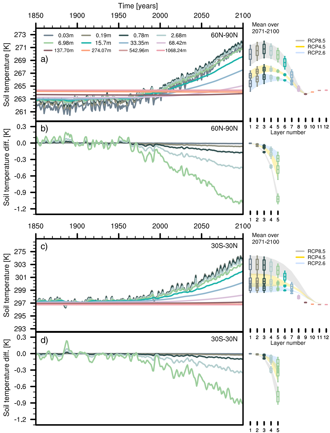
FIG. 8. As in Fig. 6, but for different latitudinal bands (see legend): (a),(b) NH high latitudes (60°–90°N) and (c),(d) intertropical regions (30°S–30°N). Note that, while the vertical scale is different for each latitudinal band, the temperature range is the same for each panel in order to make them comparable.
