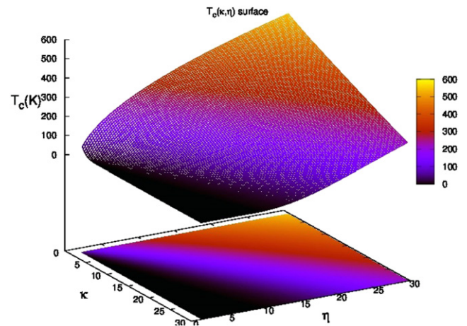
Figure 2. Plot as in figure 1 of T_c(\kappa, \eta) taken from the AD equation (origin is at far left) emphasizing very large values of the arguments. As in figure 1 T_c is normalized to values for \text{H}_3\text{S} ( T_c = 200 K). The large values of T_c lie along the \eta = N(0)I^2 axis; the lattice stiffness \kappa = M\Omega^2 is of somewhat secondary importance, but of course important for stability of the lattice.
