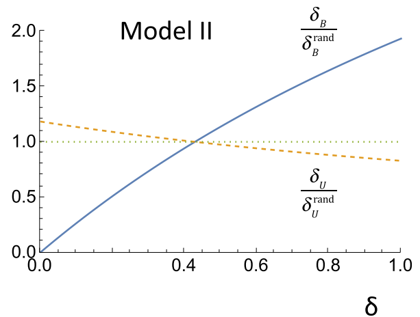
Fig. 10. \delta_U \equiv \frac{\mu_{UU}}{\mu_{UB}} and \delta_B \equiv \frac{\mu_{BB}}{\mu_{BU}} , defined in terms of the average number of links between biased and unbiased communities, rescaled by the values they adopt in a random network where links are not determined by the preference of the agents, \delta_B^{\text{rand}} = \frac{\gamma}{1-\gamma} , \delta_U^{\text{rand}} = \frac{1-\gamma}{\gamma} , as a function of \delta = \frac{\mu_{BB}}{\mu_{UU}} for both model I and II, defined in the main text. Values of \delta_B larger (resp. smaller) than \delta_B^{\text{rand}} indicate a closed (resp. open) biased community, and similarly for the unbiased community. We consider a minority fraction \gamma = 0.3 of biased agents.
