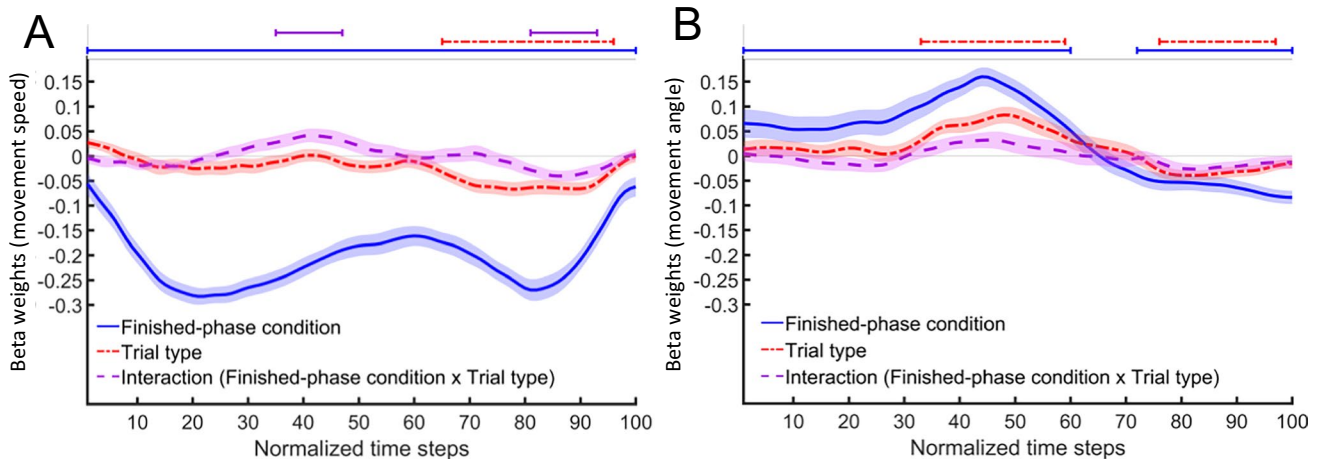
Fig. 4 Results of continuous regression analyses on mouse movement in PM_{REPEATED} vs. oddball trials (dash-dotted line) and in PM_{REPEATED} vs. ongoing-task only condition (solid line) with the dashed line showing the interaction of condition and trial type. Continuous regression analyses were performed on speed (a) and angle (b) of mouse movement. Lines above the graphs indicate segments of beta weights that differ significantly from zero (t-test, a minimum of ten consecutive significant time steps). Confidence areas indicate standard errors of beta weights. The positive/negative characteristics describe the direction of effects. Positive beta weights signify larger values in PM_{REPEATED} than in oddball trials (dash-dotted line),
