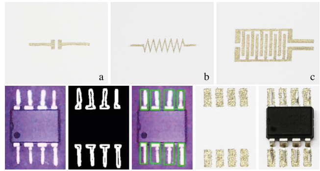
Figure 14: Top: (from left to right) Footprint for a 2835 component, printed resistor, moisture sensor. Bottom: IC footprints can be created on-the-fly by scanning the component to be used. (From left to right) RGB image, detected outlines, generated footprint, printed footprint and printed footprint together with surface-mount IC.
