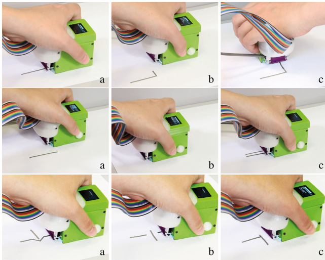
Figure 13: Top: Printing angle: a) defining the size of angle on-the-fly, b) printing the angle, c) continuing the trace. Middle: Printing a trace parallel to a previously printed trace: a) selecting a previously printed trace, b) placing the printer on existing trace and defining the distance between the traces, c) printing the new trace. Bottom: Various actions after detecting a previously printed trace: a) routing around the detected trace if there is enough space, b) stop printing before reaching to the trace and continuing after the detected trace, c) forcing to connect to the detected trace.
