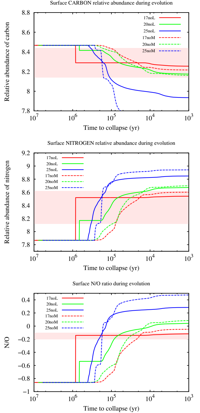
Figure 6. Same as figure 2, but for 17, 20, and 25 M_{\odot} non-rotating models.
