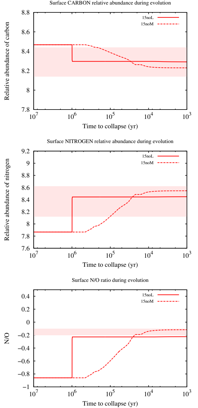
Figure 2. Relative surface abundance of carbon, nitrogen, and the surface N/O ratio for 15 M_{\odot} models with no rotation. Top panel is carbon, middle panel nitrogen, and bottom panel the N/O ratio. “Time to collapse” refers to the time until the end of the evolution. The region shaded in red indicates the adopted observational constraints as given in section 2. Solid lines are L_A overshoot models, while dashed lines are M_A overshoot models.
