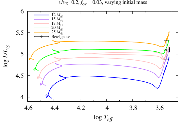
Figure 5. Evolution tracks for 12 to 25 M_{\odot} models with v/v_K = 0.2 and L_A .
