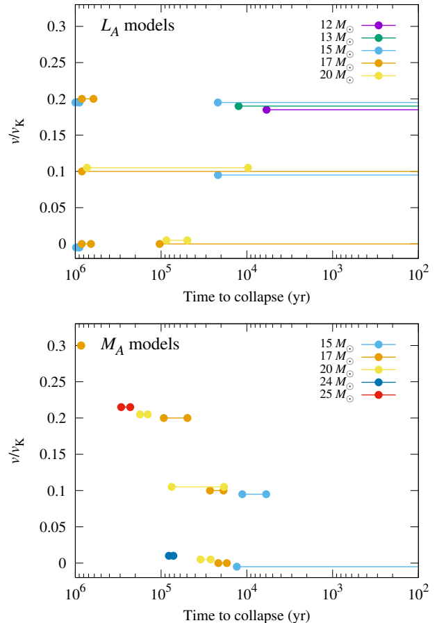
Figure 7. The timing of the fit for certain models with varying initial parameters, shown as a comparison.
