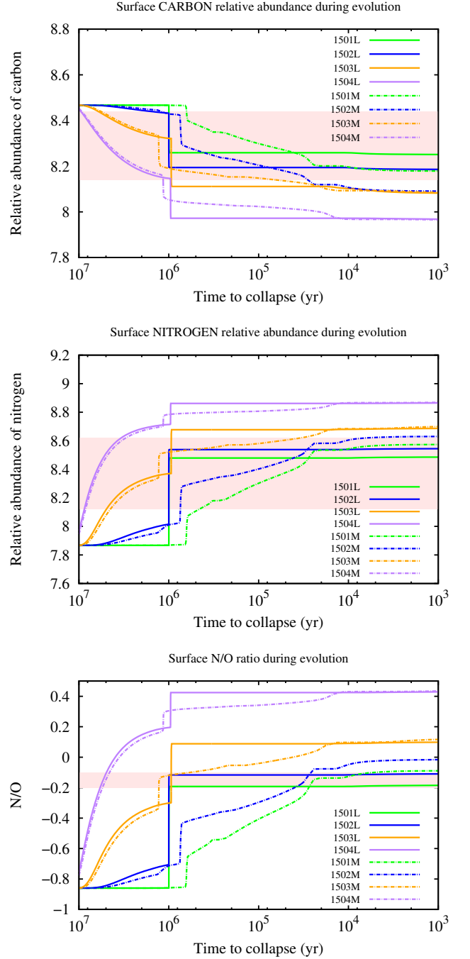
Figure 4. Same as figure 2, but for 15 M_{\odot} models with varying initial rotation.
