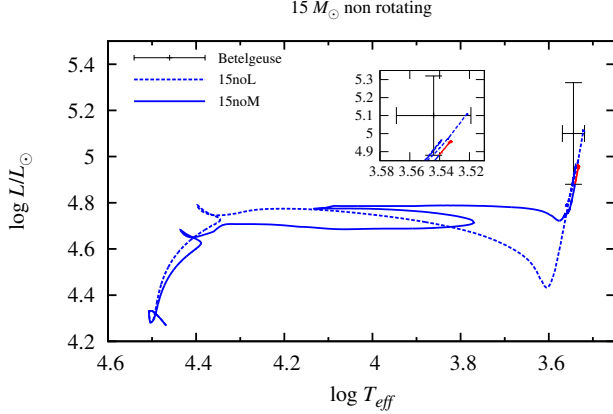
Figure 1. Evolution tracks for the non-rotating 15 M_{\odot} models applied with different overshoot parameters. The inset plot is zoomed in and focused on the observed HR diagram position of Betelgeuse. The error bars are the same as those in Dolan et al. (2016). The period where the model satisfies Betelgeuse’s observational constraints are indicated in red.
