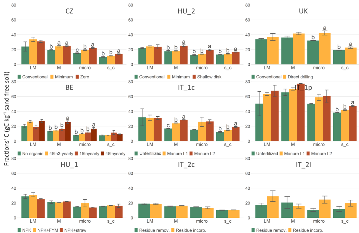
Figure 6. The SOC content in each aggregate fraction expressed in a sand free soil for each study. (Codes and description of the practices are presented in Table 1.) The error bars represent the standard error. Within an experiment and fraction, bars with a different letter differ significantly according to Tukey's test ( p < 0.05 ).
