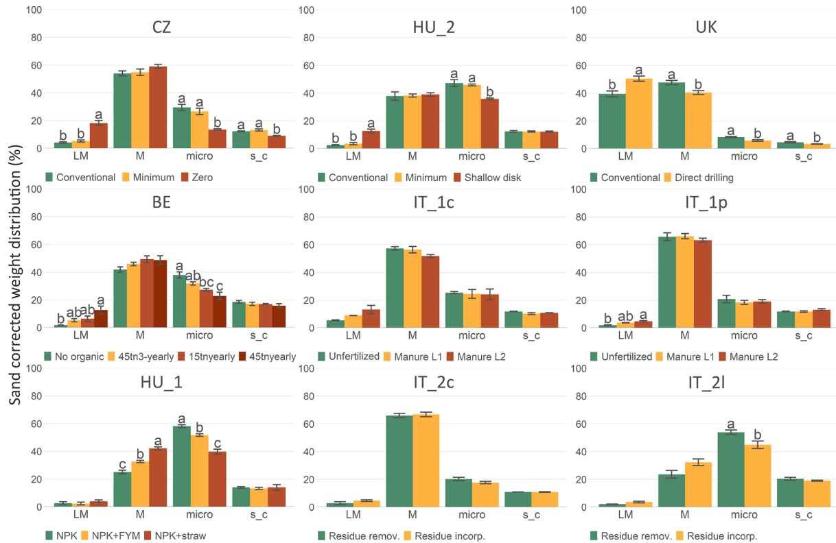
Figure 5. Weight distribution of sand free aggregate fractions for each study site. (Codes and description of the practices are presented in Table 1.) The error bars represent the standard error. Within an experiment and fraction, bars with a different letter differ significantly according to Tukey's test ( p < 0.05 ).
