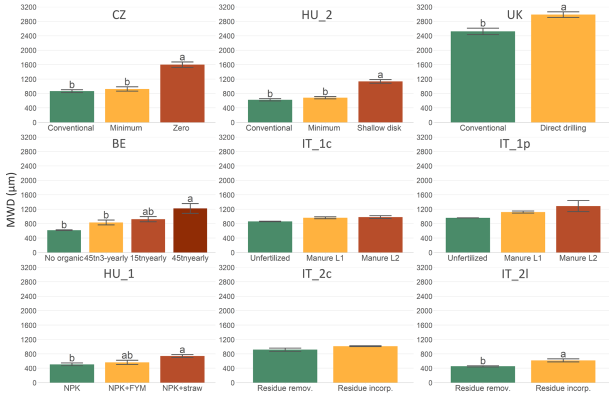
Figure 3. Mean weight diameter (MWD) of sand free aggregates in the topsoil (0–15 cm) for each study site. (See also Table 1 for the codes and a description of the treatments.) The error bars represent the standard error. Within an experiment, bars with a different letter differ significantly according to Tukey's test ( p < 0.05 ).
