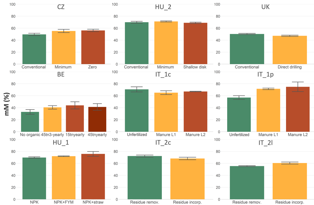
Figure A2. Mass percentage of the occluded microaggregates within the macroaggregates (mM). The mM mass is expressed as percentage of macroaggregates. The error bars represent the standard error. Within an experiment, bars with a different letter differ significantly according to Tukey’s test ( p < 0.05 ).
