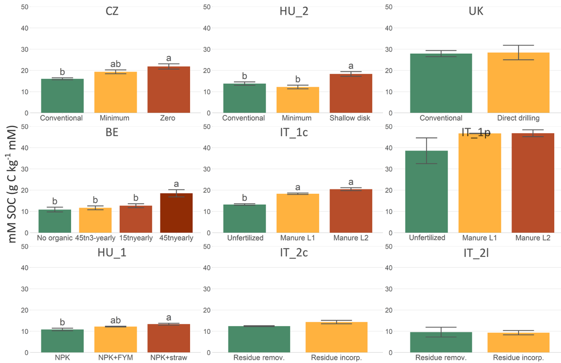
Figure 7. The SOC content in the microaggregates held within the macroaggregates fraction (mM-C). (Codes and description of the practices are presented in Table 1.) The OC content is expressed in g C per kg of occluded microaggregates. The error bars represent the standard error. Within an experiment, bars with a different letter differ significantly according to Tukey's test ( p < 0.05 ).
