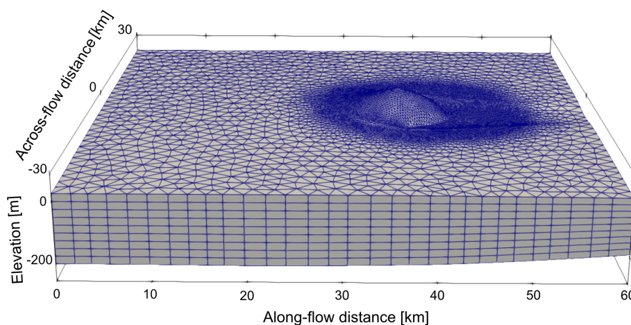
Figure 2. Shown is the mesh resolution. In the horizontal, the mesh is unstructured and has a resolution of 350 m in the area surrounding the ice rise or ice rumples. The background resolution (of the surrounding ice shelf) is 2000 m. The mesh is extruded in the vertical with 10 layers. Note that the geometry is exaggerated by a factor of 30 in the vertical direction.
