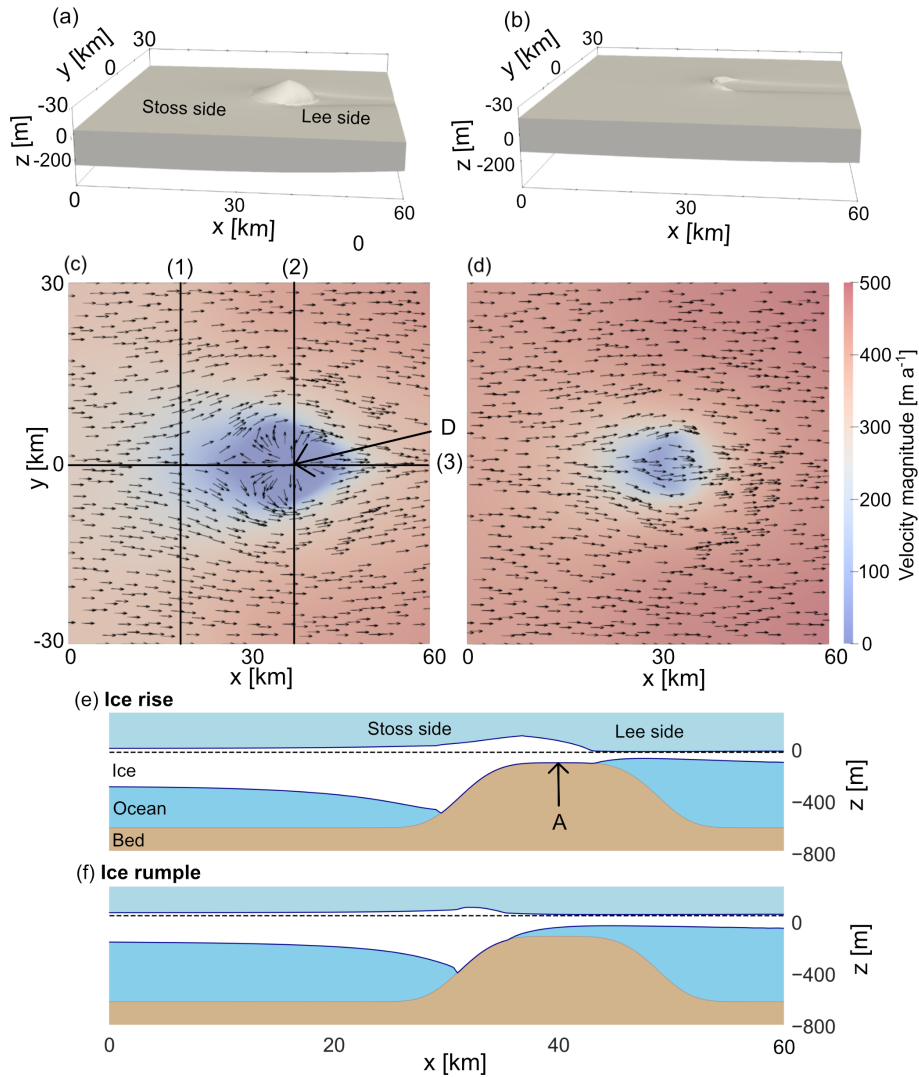
Figure 1. The 60 km × 60 km model domain is shown in the case of (a) an ice rise and (b) an ice rumples. A corresponding bird’s eye view in (c) and (d) shows the surface velocity magnitude colour-coded and the ice flow direction with arrows. Corresponding along-flow cross-sections are shown in (e) and (f). Sea level is at an elevation of 0 m in the case of the ice rise and 80 m in the case of the ice rumples. In (c), (1), (2), and (3) indicate cross-sections used for analysis, and D is the ice rise dome. Both (2) and (3) are cross-sections through the ice rise dome. In (e), A marks the highest point of the bed anomaly. The x direction corresponds with the along-flow direction, the y direction corresponds with the across-flow direction, and the z direction corresponds with the elevation.
