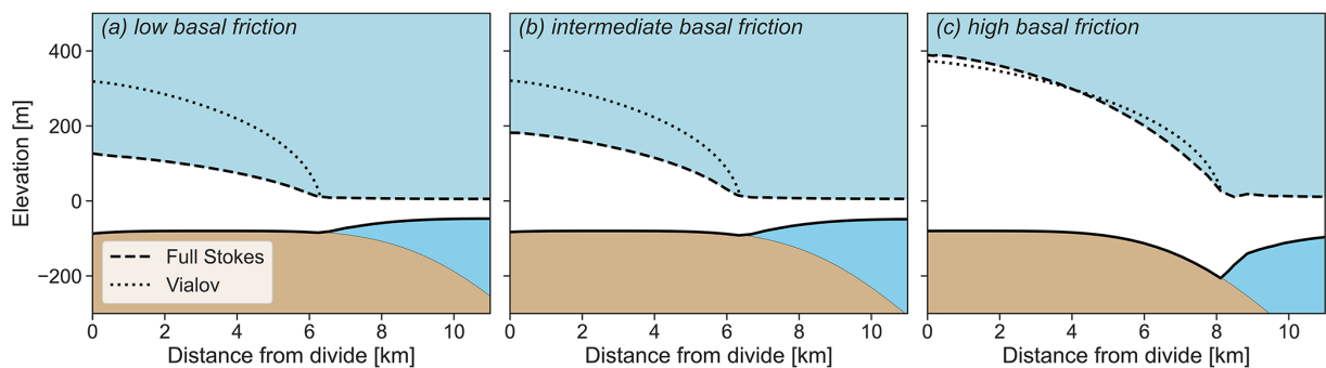
Figure 7. Cross-sections of the full Stokes simulations at t = 2000 years in the case of the (a) low-, (b) the intermediate-, and (c) the high-basal-friction coefficient. Using a reference point on the ice surface at the grounding line, a Vialov profile is calculated and plotted.
