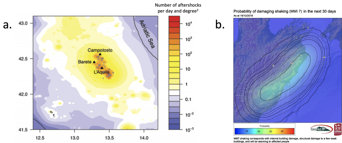
Figure 1. Two examples of aftershock forecasts. (a) A map showing the expected daily number of aftershocks above magnitude 2.0 several weeks after the L'Aquila, Italy, earthquake of 2006 (reprinted from Murru et al., 2015). (b) A map showing the forecasted probability of a damaging aftershock (defined as having a Modified Mercalli Intensity – MMI – score above 7) in the month following the Kaikōura, New Zealand, earthquake of 2016, released to the public by New Zealand's GNS Science (reprinted from Becker et al., 2020). As damaging earthquakes are rare, even probabilities above 10 % may constitute a significant risk, though disentangling the uncertainty around this forecasted probability is not possible from this map.
