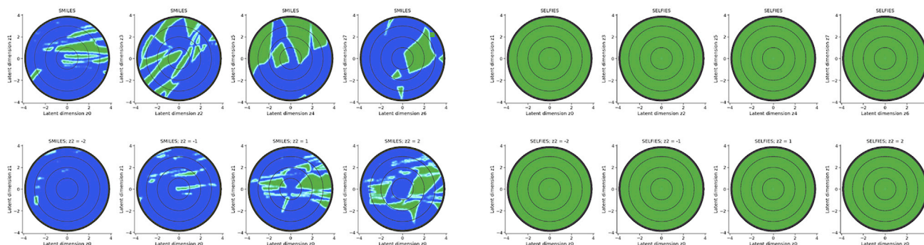
Figure 3. Decoding points from the internal representation (latent space) of a variational autoencoder (VAE) Green stands for valid and blue for invalid molecules. The left image is trained using SMILES strings, most of its latent space representing invalid molecular strings. The right image shows the latent space of a VAE trained with SELFIES. Every point stands for a physically meaningful molecule. Figure from Krenn et al. 27
