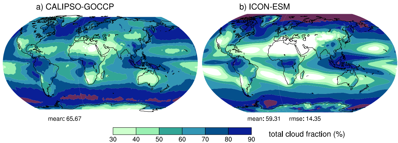
Figure 8. Total cloud fraction (%) (a) from the CALIPSO-GOCCP observations averaged over 2007–2019 and (b) from the ICON-ESM historical simulation averaged over 1979–2014. Numbers below the panels indicate global means and root mean square difference between simulation and observation.
