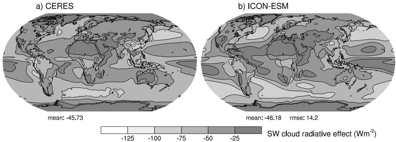
Figure 10. Short wave cloud radiative effect ( \text{Wm}^{-2} ) from (a) CERES observations averaged over 2001–2020 and (b) from the ICON-ESM historical simulation averaged over 1979–2014. Numbers below the panels indicate global means and root mean square difference between simulation and observation.
