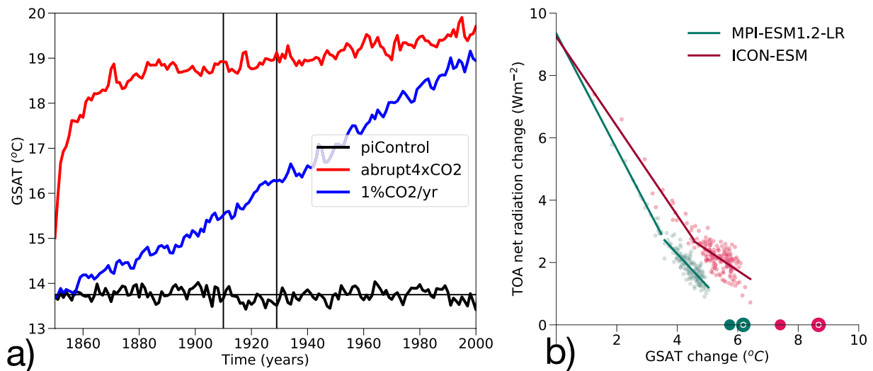
Figure 28. Estimating the Transient Climate Response (TCR) and Equilibrium Climate Sensitivity (ECS) from idealized DECK experiments. (a) Evolution of global surface air temperature in the 1pctCO 2 (blue) and abrupt4XCO 2 (red) together with the piControl experiment (black). Vertical lines indicate the period for the TCR calculation and (b) regression analyses to estimate ECS in ICON-ESM (dark red) and in MPI-ESM1.2. The small dots on the horizontal axis indicate twice the ECS based on a regression using the first 150 years following Gregory et al. (2004). The bigger dots show the respective intersection of the regression based on years 20–200.
