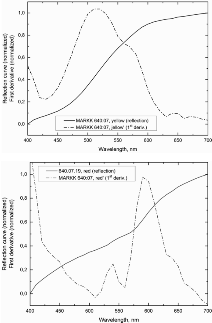
FIGURES 26–27 VIS spectra with corresponding first derivatives of the yellow (top) and red organic dye (bottom). The comparison of the reflection curves (local minima and maxima, inflection points) with corresponding references allows the assignment of gamboge as a yellow dye and carmine as a red dye.
