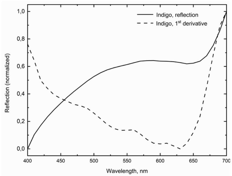
FIGURES 19–20 VIS spectra of indigo and ultramarine (nineteenth-century geomancy map, (MARKK 85.48:2); Chinese pilgrimage map Wutaishan sheng jing quan tu 五臺山聖境全圖, (MARKK XX SOAS 408)).
