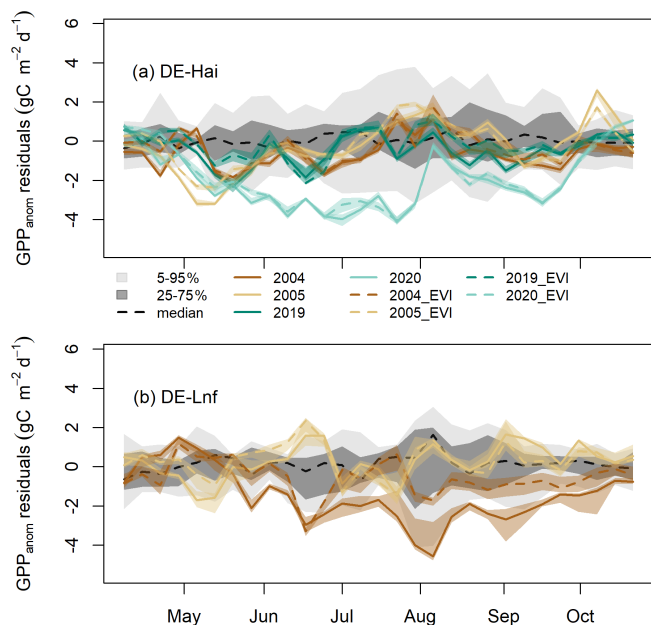
Figure 5. Residuals of GPP anomalies from RF and RF_{EVI} (see Sect. 3.6) in legacy years at (a) DE-Hai and (b) DE-Lnf. Residuals of GPP anomalies are characterised by observed minus predicted GPP anomalies ( GPP_{anom} residuals). The coloured lines and bands show the median and 5th–95th percentile GPP_{anom} residuals of ensemble model runs (see Sect. 3.4), respectively. The solid and dashed lines show the residuals based on RF and RF_{EVI} , respectively. The model uncertainties from RF_{EVI} (dark and light grey shaded areas, respectively) are characterised by the 25th–75th and 5th–95th quantile ranges of GPP_{anom} residuals in non-legacy years. The black dashed line was the median of GPP_{anom} residuals from RF_{EVI} in non-legacy years. The ticks denote the start of each month. Figure S4 shows the results for April–June and August–October at DE-Hai in more detail.
