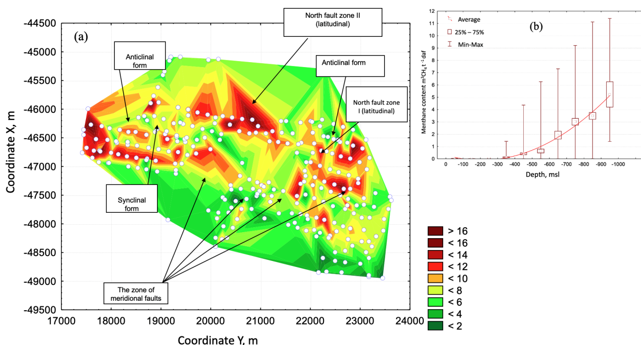
Figure 2. Methane content ( M_c ) variability depending on depth and across the deposit exemplarily shown for the Brzeszcze coal mine. (a) Wafer chart of the methane content isolines within the deposit 352 in the Brzeszcze coal mine in a two-dimensional space with marked disturbances of the geological structure. White dots indicate methane content measurement points. The disorders observed based on the geological structure of the deposit are described in square boxes; x and y are the coordinates. (b) Frame chart of methane content variability at individual depth intervals in the Rydułtowy coal mine with significant mean values as a midpoint. The box corresponds to the range of results from 25 % to 75 %, while the whiskers represent the minimum and maximum values.
