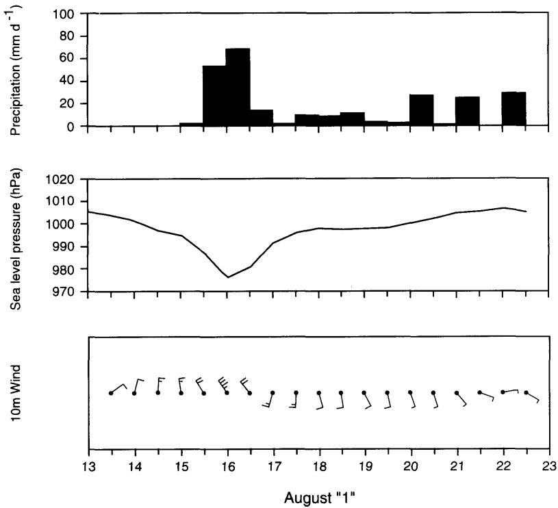
Fig. 2. Metogram for Fu-Chou (Fukien, China) showing precipitation, surface pressure and 10 m wind for every 12 h from 13 August to 22 August, year 1 of the simulation.
