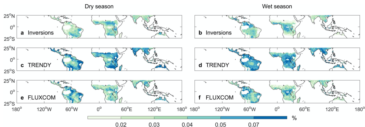
Supplementary Figure 3 Spatial distribution of the ratio between the standard deviation of NEE during the dry or wet season and the standard deviation of global annual NEE.
