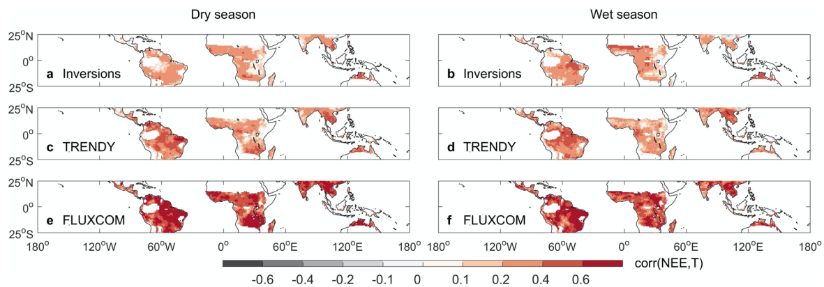
Supplementary Figure 11 Spatial distribution of correlation between NEE and T during the dry and wet seasons. NEE is estimated by atmospheric inversions ( a, b ), DGVMs from TRENDY in simulation S2 (NEE output) ( c, d ) and FLUXCOM models ( e, f ). The left column indicates the correlation of NEE with T during the dry season and the right column indicates the correlation with T during the wet season.
