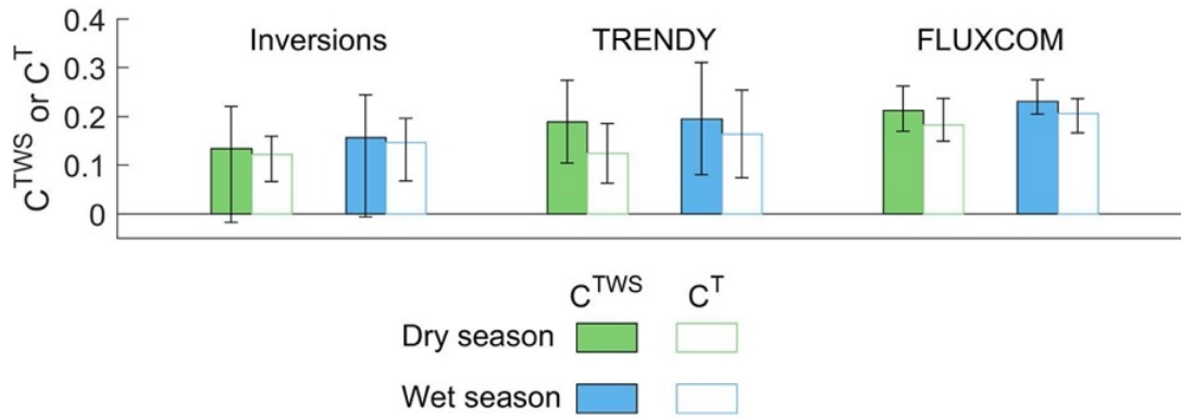
Supplementary Figure 1 Contribution of tropical NEE during the dry and wet seasons to the global r_{TWS} and r_T . Solid bars are the contribution to the global r_{TWS} ( C^{TWS} ) while open bars are the contribution to the global r_T ( C^T ). Green bars indicate the C^{TWS} or C^T during the dry season while blue bars indicate the C^{TWS} or C^T during the wet season. NEE is estimated by atmospheric inversions, DGVMs from TRENDY in simulation S2 (NEE output) and FLUXCOM models. For atmospheric inversions and FLUXCOM models, the error bars indicate the range of models while for DGVMs from TRENDY, the error bars indicate the 1- \sigma inter-model spread.
