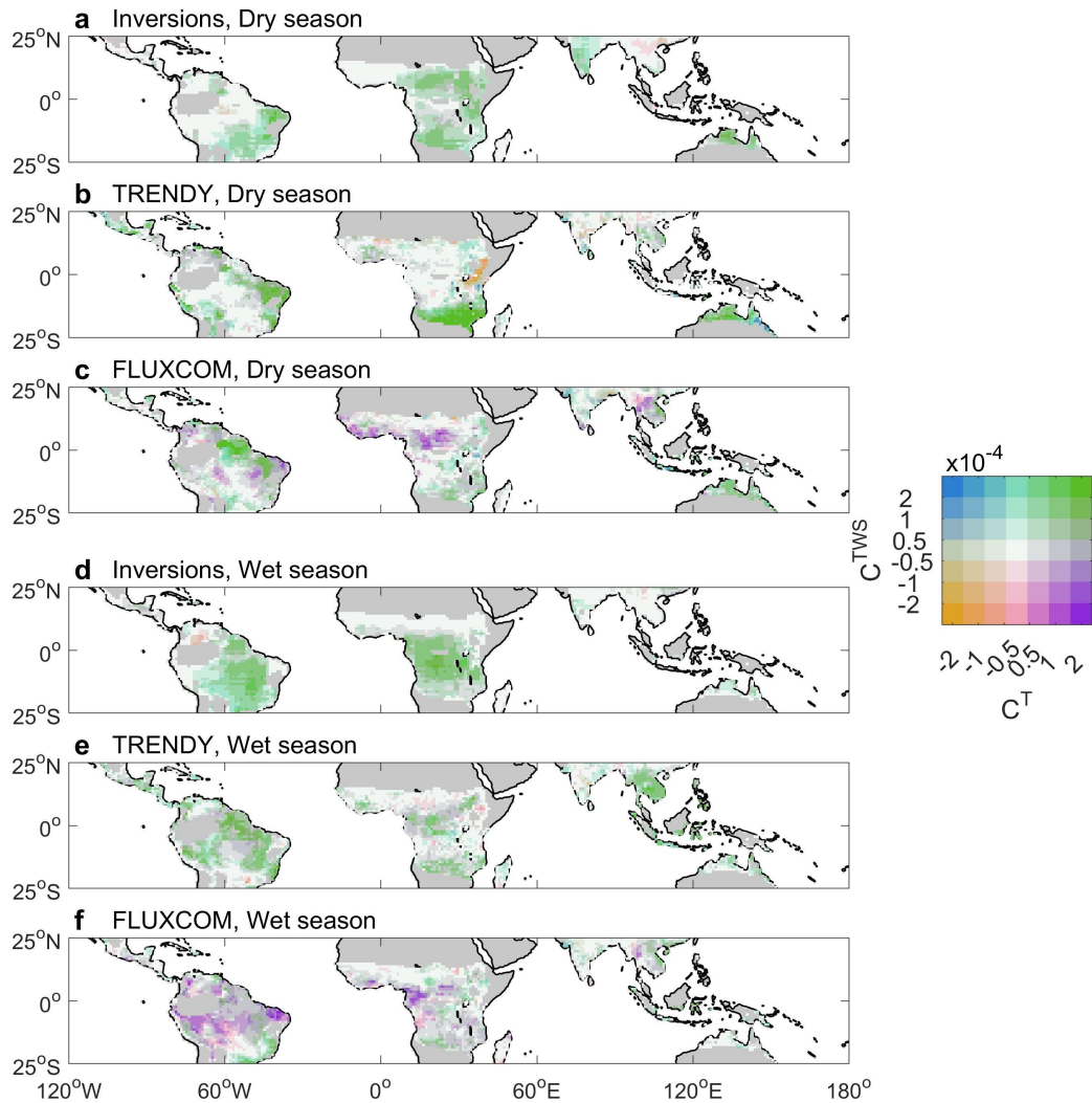
Supplementary Figure 9 Spatial distribution of the C^{TWS} and C^T in tropics during the dry and wet seasons. NEE is estimated by atmospheric inversions ( a , d ), DGVMs from TRENDY in simulation S2 (NEE output) ( b , e ), and FLUXCOM models ( c , f ). The pixels where there is only dry or only wet season within a year are excluded. Note that in panels a and d , TWS is reconstructed based on GRACE observations. By contrast, in panels b and e , simulated soil moisture in DGVMs from TRENDY is used as TWS while in panels c and f , water availability index (WAI) in FLUXCOM models is used.
