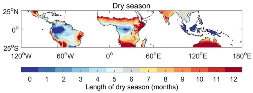
Supplementary Figure 5 Map in length of dry season for each pixel.
