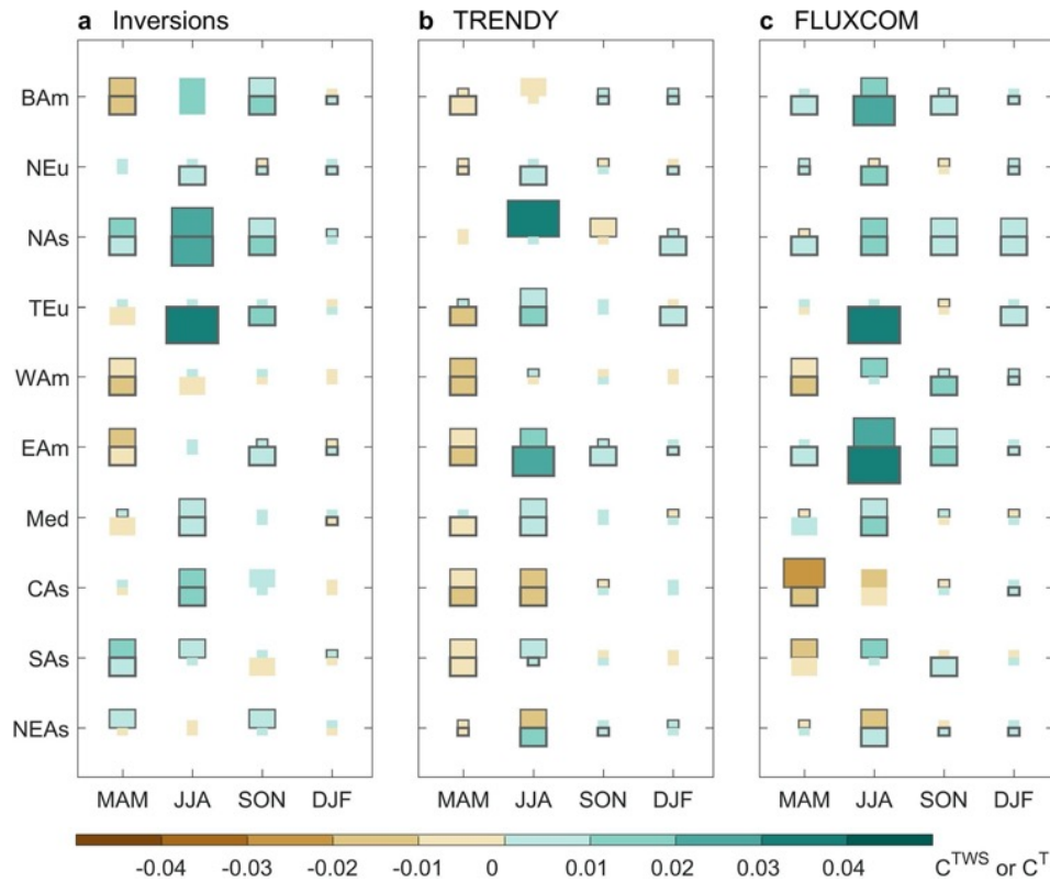
Supplementary Figure 6 C^{TWS} and C^T in northern extra-tropical sub-regions during four seasons. NEE is estimated by atmospheric inversions (a), DGVMs from TRENDY in simulation S2 (NEE output) (b), and FLUXCOM models (c). For each season and each region, two rectangles ( C^{TWS} in the top and C^T in the bottom) are shown. The larger rectangles indicate the higher absolute values of the C^{TWS} or C^T . The four seasons are boreal spring (MAM, March–May), summer (JJA, June–August), autumn (SON, September–November), and winter (DJF, December and January–February). Northern Hemisphere (NH, >25^\circ\text{N} ) is divided into ten sub-regions (see map in Fig. 6). BAm: Boreal America, NEu: North Europe, NAs: North Asia, TEu: Temperate Europe, WAm: Western North America, EAm: Eastern North America, Med: Mediterranean, CAs: Central Asia, SAs: South Asia and subtropical China, and NEAs: Northern East Asia. For atmospheric inversions and FLUXCOM models, black edges of the rectangles indicate that the signs of the C^{TWS} or C^T are the same among all models. For DGVMs, black edges of the rectangles indicate that the signs of C^{TWS} or C^T derived from more than 10 out of 14 models are consistent with those from the model ensemble mean.
