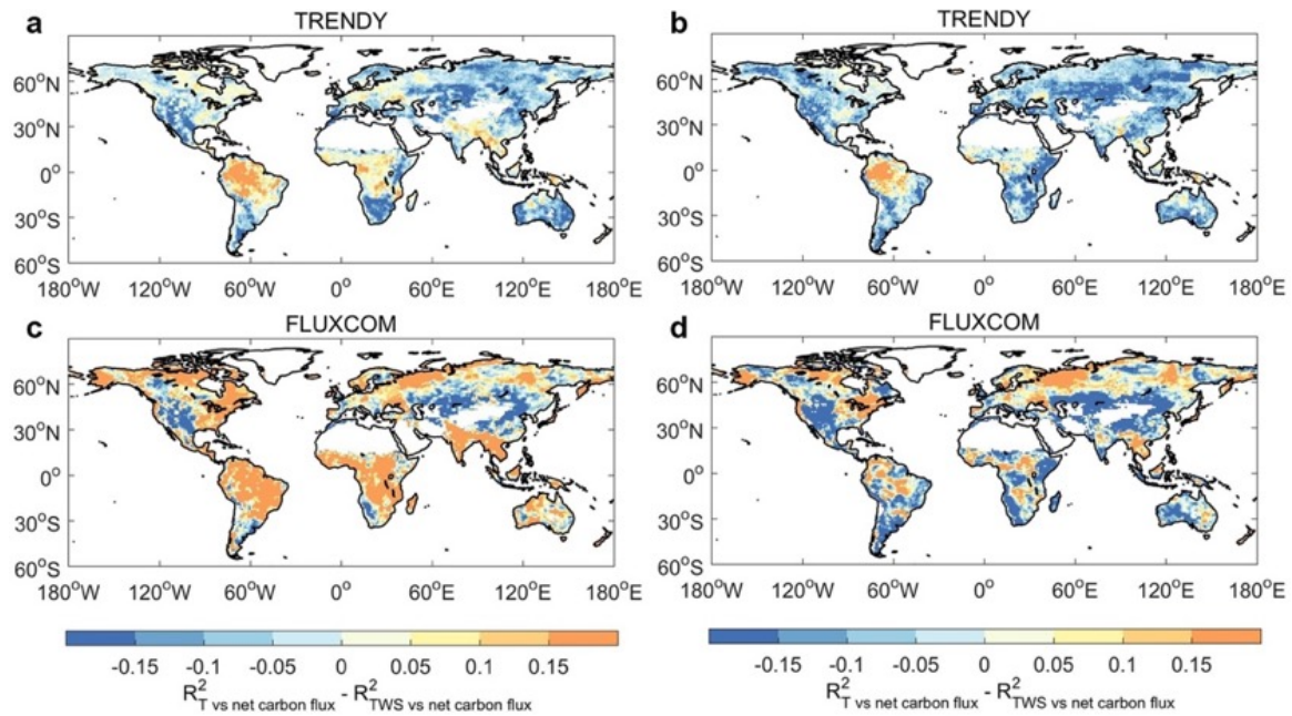
Supplementary Figure 7 Spatial distribution of difference between R^2 of NEE with T and that with water availability. Yellow pixels indicate NEE_{IAV} is more correlated to T than to water availability (represented by TWS) while blue pixels indicate more correlated to water availability. Note that in panels a and c , water availability is from GRACE TWS reconstruction and in panels b and d , water availability is simulated soil moisture by DGVMs from TRENDY and Water Availability Index (WAI) in FLUXCOM models, respectively.
