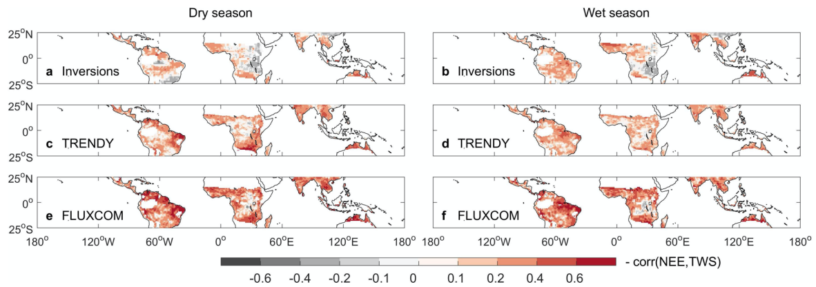
Supplementary Figure 4 Spatial distribution of correlation between NEE and TWS during the dry and wet seasons. NEE is estimated by atmospheric inversions ( a, b ), DGVMs from TRENDY in simulation S2 (NEE output) ( c, d ) and FLUXCOM models ( e, f ). The left column indicates the correlation of NEE to TWS during the dry season and the right column indicates the correlation to TWS during the wet season. Note that the correlation coefficient is shown with the opposite sign.
