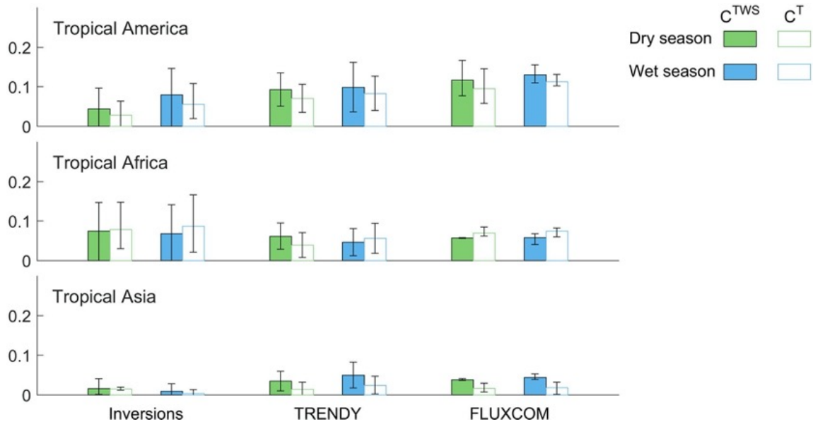
Supplementary Figure 2 Contribution of NEE in three tropical continents during the dry and wet seasons to the global r_{TWS} and r_T . Three tropical continents are tropical America, tropical Africa and tropical Asia, and the latter includes northern Australia. Solid bars are the contribution to the global r_{TWS} ( C^{TWS} ) while open bars are the contribution to the global r_T ( C^T ). Green bars indicate the C^{TWS} or C^T during the dry season while blue bars indicate the C^{TWS} or C^T during the wet season. NEE is estimated by atmospheric inversions, DGVMs from TRENDY in simulation S2 (NEE output) and FLUXCOM models. For atmospheric inversions and FLUXCOM models, the error bars indicate the range of models while for DGVMs from TRENDY, the error bars indicate the 1- \sigma inter-model spread.
