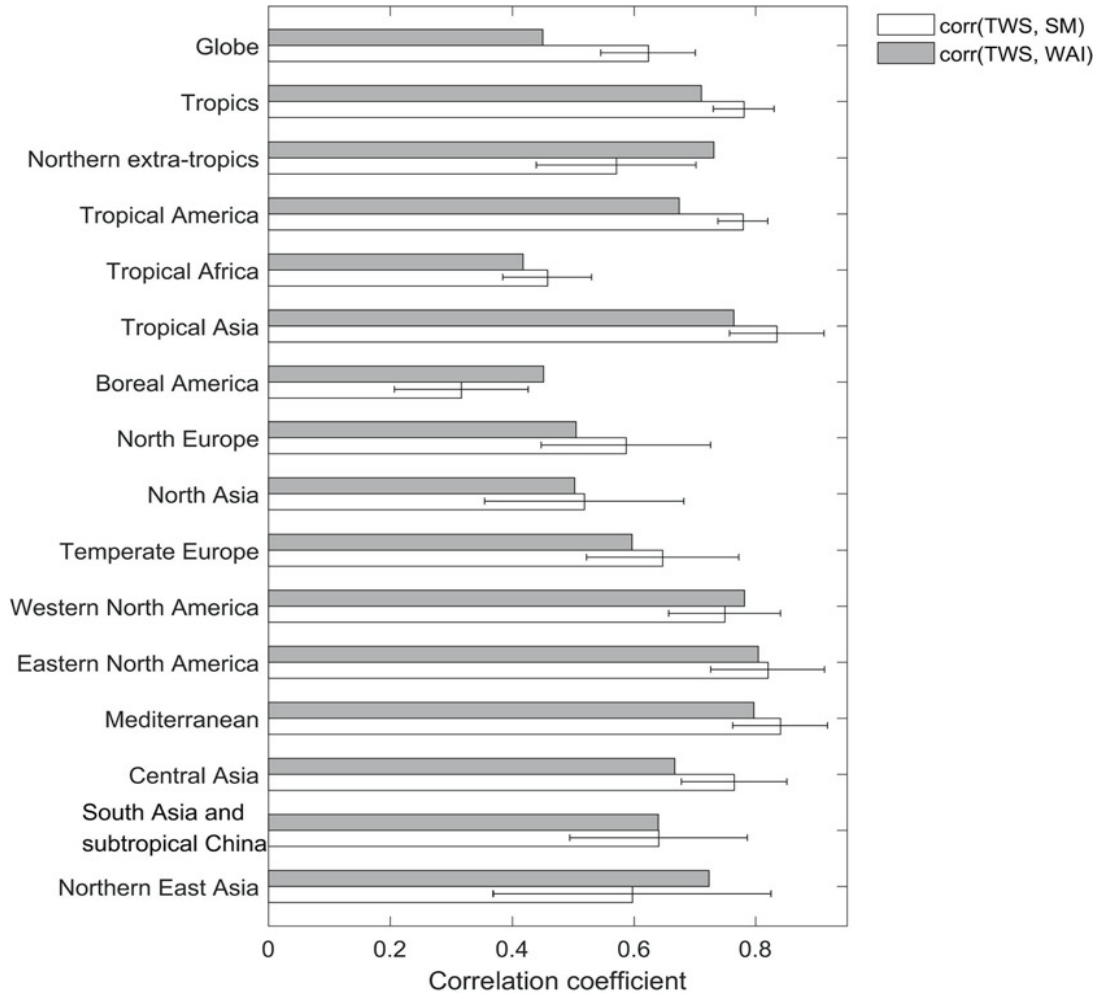
Supplementary Figure 10 Correlation coefficient between the reconstructed TWS based on GRACE observations and DGVMs-simulated soil moisture (SM) or Water Availability Index (WAI) used in FLUXCOM models. Error bars for correlation coefficient between reconstructed TWS and DGVMs-simulated soil moisture indicate the 1- \sigma inter-model spread.
