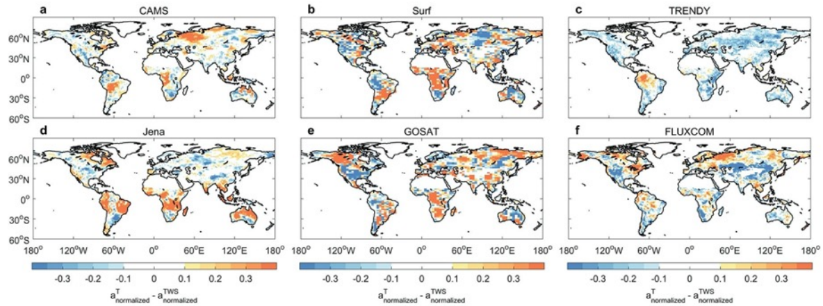
Supplementary Figure 8 Spatial distribution of difference between sensitivity of net carbon flux to T and that to water availability. The net carbon flux is estimated by atmospheric inversions ( a , b , d , e ), DGVMs from TRENDY project ( c ), and FLUXCOM models ( f ). Atmospheric inversions assimilate surface measurements (CAMS, Jena and Surf; see Methods) and total column CO 2 dry air mole fraction retrievals from the Japanese Greenhouse gases Observing SATellite (GOSAT). For comparison, the inversions based on surface observations (Surf) and GOSAT data have the same time span 2010–2016. Note that net carbon flux estimated by DGVMs from TRENDY ( c ) is the NBP output in simulation S3 (see Methods). Water availability is TWS reconstructed from GRACE observations when estimating the sensitivity of atmospheric inversed carbon flux to water availability. In the estimation of sensitivity of modeled carbon flux from DGVMs and FLUXCOM models, water availability is simulated soil moisture by DGVMs and Water Availability Index (WAI) in FLUXCOM models, respectively. Note that when calculating the sensitivities, all variables were normalized by the standard deviation, and then the absolute values of the sensitivities were used.
