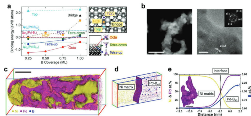
Figure 1. DFT calculation and high-resolution microscopy and microanalysis of B-incorporating Pd nanomaterials. a) Binding energies E_b of B adsorbates at the Pd(111) surface and subsurface for several adsorbate coverages in the range from 0.25 to 1 ML. Each colored solid line corresponds to a different B binding site. Different chemical potentials of B, ( \mu_r gives the reductant to precursor ratio) of the considered synthesis conditions are shown as horizontal colored dashed lines. The possible binding sites at the surface are shown (top) in top-view and at the subsurface (bottom) in a side-view. The white (gray) balls represent surface (subsurface) Pd atoms. The p(2 \times 2) surface unit cells are indicated by black solid lines. b) HAADF-STEM (left) and HR-TEM (right) images of as-synthesized Pd- \text{B}_{40} nanoparticles. Scale bars are 50 and 5 nm, respectively. The inset shows the [110] zone axis in a FFT pattern. c) 3D atom maps of Pd- \text{B}_{40} fully embedded in a Ni matrix as indicated by the Ni iso-surfaces. Scale bar: 20 nm. d) Extracted region ( 2 \times 5 \times 10 \text{ nm}^3 ) of interest along the Pd/Ni interface. Yellow, purple, and blue dots mark the reconstructed positions of Ni, Pd, and B atoms, respectively. e) 1D compositional profiles of elements across Pd- \text{B}_{40} nanoparticles. The inset image shows a 3D reconstruction of the Pd- \text{B}_{40} . Scale bar: 20 nm.
