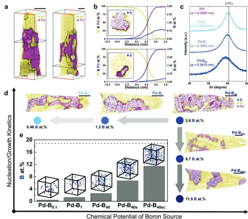
Figure 2. Controlling the magnitude of B content in Pd nanoparticles by synthesis. a ) 3D atom maps of (left) Pd-B 1 and (right) Pd-B 0.1 nanoparticles embedded in a Ni matrix. b ) 1D compositional profile along the Pd/Ni interface for (top) Pd-B 1 and (bottom) Pd-B 0.1 . Each inset shows the corresponding top-view tomogram. c ) XRD patterns of Pd-B x samples synthesized with different reductant concentrations. The dotted line represents the corresponding (111) peak position. d ) Schematic plot of the chemical potential of the boron source versus Pd-B x nanoparticle growth kinetics. Insets show tomograms (1 nm thin slice along the x-axis) of each reconstructed Pd nanoparticle sample. All scale bars are 20 nm. e ) B atomic content in Pd-B 0.1 , Pd-B 1 , Pd-B 40 , Pd-B 40s , and Pd-B 40sc samples. The dotted line represents the maximum B content that FCC Pd metal can absorb without undergoing a phase transformation. [59] The insets show the extracted cuboidal region of interest (5 × 5 × 5 nm 3 ) of each as-synthesized Pd-B x nanoparticle.
