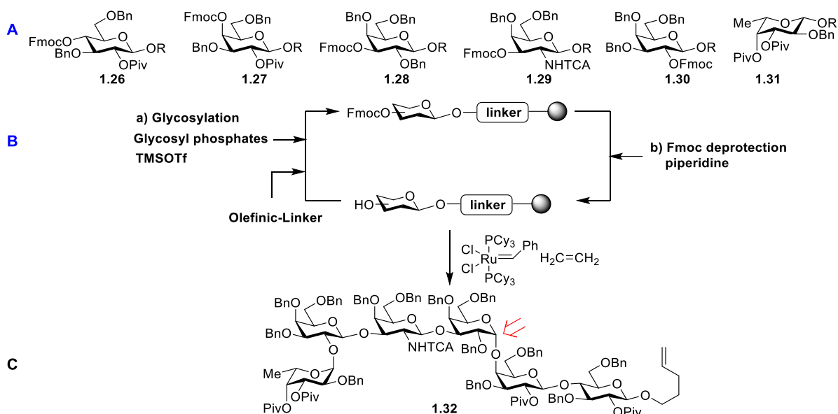
Figure 1.12 Automated synthesis of Globo-H. 32d
