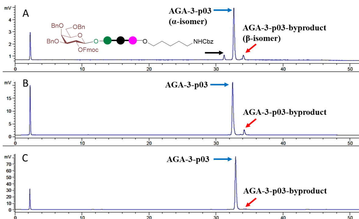
Figure 3.04. NP-HPLC of the protected pentasaccharide AGA-3-p03 . HPLC was performed using Luna Silica. Conditions: eluents: hexane/ethyl acetate; gradient: 20% (5 min) → 45% (in 25 min) → 100% (in 5 min) at a rate 1 mL/min; detection: ELSD.
