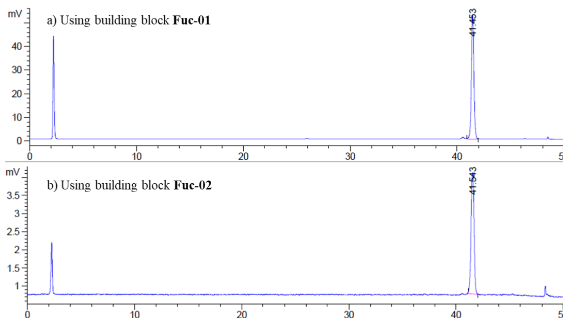
LC-MS of H-type II using fucose building block Fuc-01 and Fuc-02 . The mixture was not separable.
