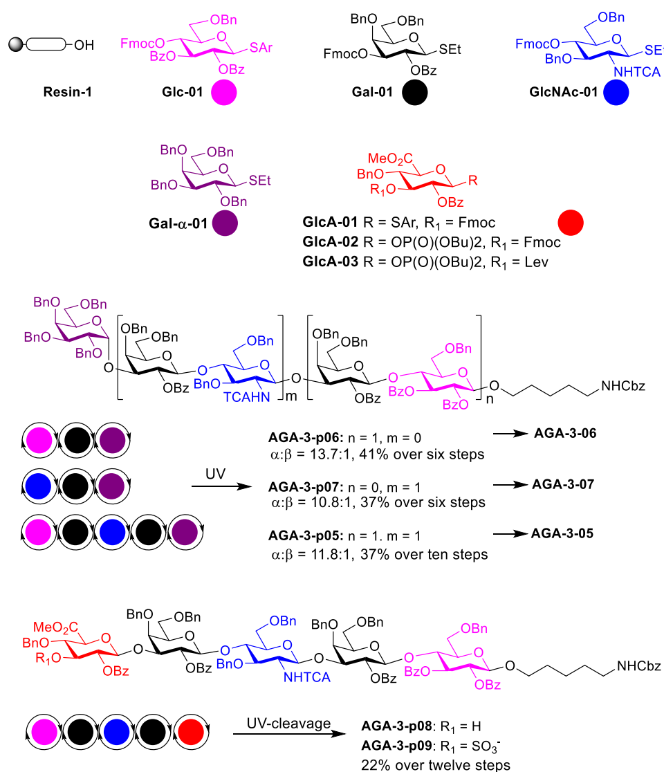
Scheme 3.02 Automated Glycan Assembly of the Protected Three \alpha -Gal epitopes AGA-3-p05 , AGA-3-p06 , and AGA-3-p07 , and Non-sulfated and Sulfated HNK-1 AGA-3-p08 and AGA-3-p09 oligosaccharide. a Reaction conditions: Glycosylation: 2 x 5 equiv of Glc-01 or GlcNAc-01 , NIS, TfOH, DCM/dioxane, -30 °C (5 min) \rightarrow -10 °C (25 min). 2 x 5 equiv of Gal-01 or Gal- \alpha -01 , NIS, TfOH, DCM/dioxane, -40 °C (5min) \rightarrow -20 °C (25 min). 2 x 7.5 equiv of GlcA-03 , TMSOTf, DCM, -10 °C (5 min) \rightarrow 0 °C (50 min); Deprotection: three cycle of 20% NEt_3 in DMF, 25 °C; three cycle of hydrazine hydrate (0.56 M in pyridine/acetic acid (v/v, 3:2); Sulfation: three cycle of 0.5 M of sulfur trioxide pyridine complex in DMF/TEA (v/v, 1:1) at 50 °C; UV-cleavage: hv (305 nm); Yields are based on resin loading and obtained by preparative HPLC (detection: ELSD)
