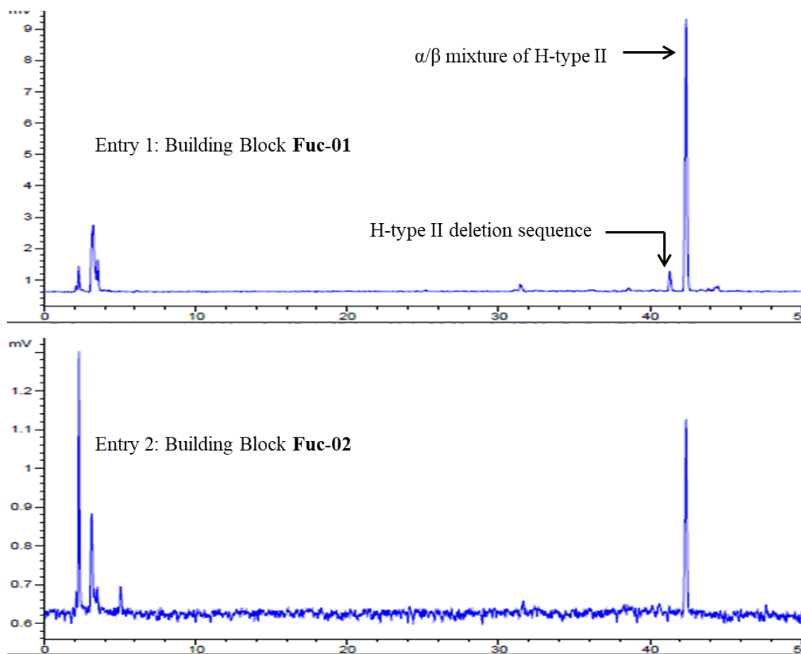
LC-MS of H-type II deletion sequence and H-type II alpha/beta mixture. Conditions: column: Luna C5 100A, (260 x 4.60 mm); flow rate: 1 mL/min; eluents: TDW/acetonitrile; gradient: 50% (5 min) 100% (in 40 min) 100% (in 5 min); detection: ELSD.
