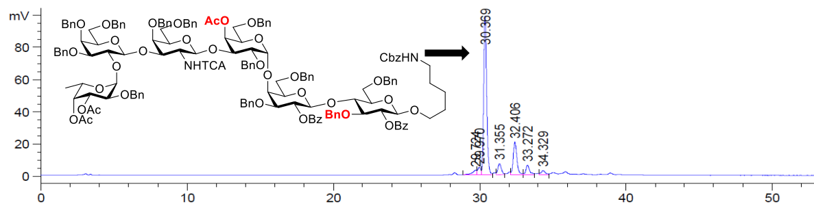
LC-MS chromatogram of AGA-4-p11.
