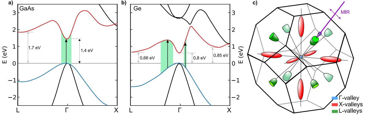
Figure 5.4: Bandstructures and Brillouin zone: a) Bandstructure of GaAs adapted from Ref. [240]. b) Bandstructure of Ge based on Ref.[241]. The bandgap values are from Ref.[242]. c) Brillouin zone of Ge and schematic illustration of the elliptic isoenergy surfaces around the \Gamma -, X- and L-valleys (adapted from Ref. [243]).
