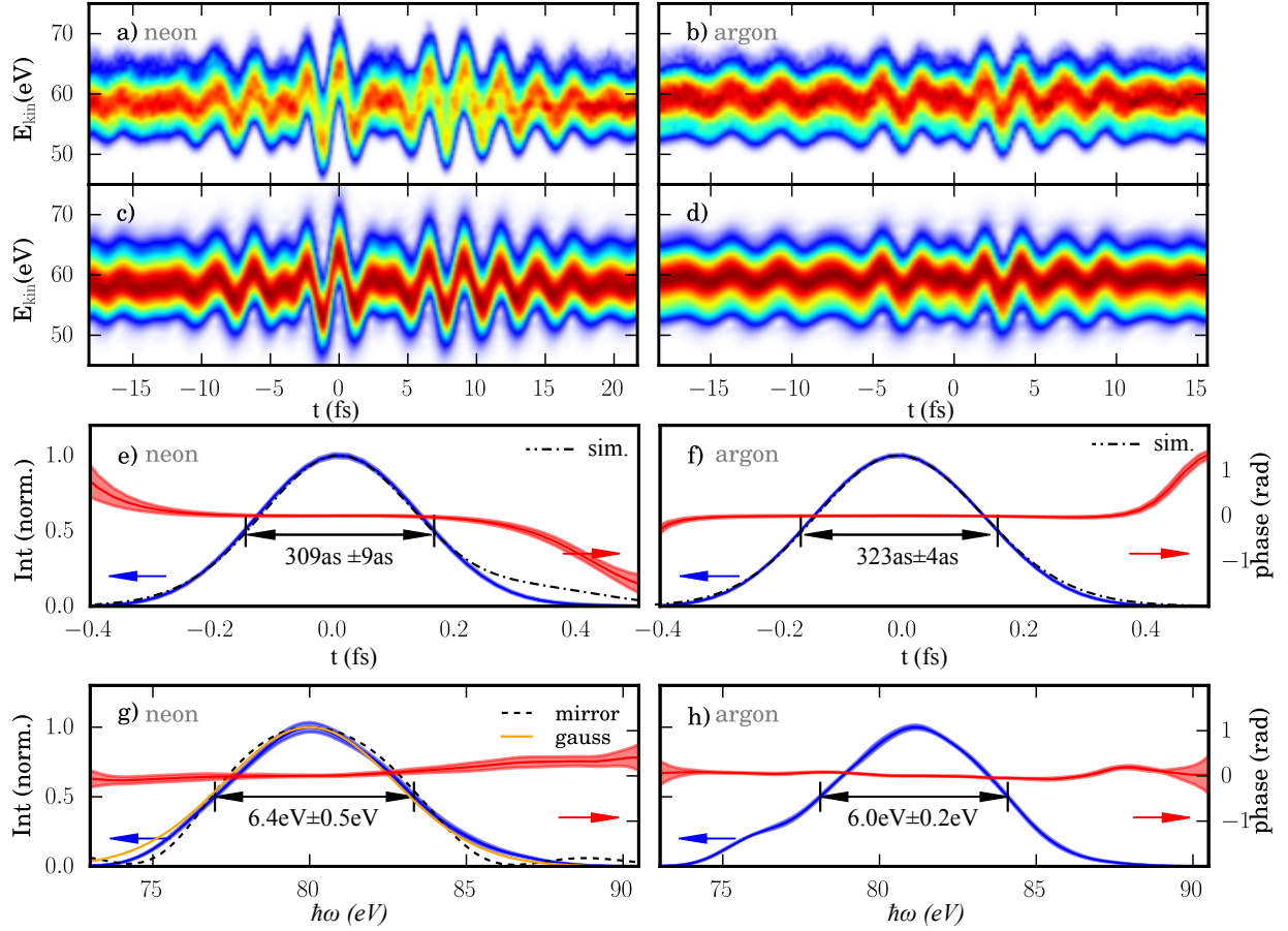
Figure 6.3: IR and XUV pulses retrieved using the pythographic reconstruction algorithm: a) and b) experimental input streaking trace and c) and d) reconstructed streaking spectrogram for neon and argon, respectively. e) and f) temporal reconstruction of the intensity (blue) and phase (red) of the isolated attosecond XUV pulses for neon and argon, respectively, and the intensity obtained from simulations (black dashed-dotted line). The colorscale is the same as in Fig. 6.2. g) and h) spectral reconstruction of the intensity (blue) and phase (red), together with the reflectivity of the XUV multilayer mirror (black dashed line, maximum reflectivity \approx 42\% ) and a Gaussian (orange line, 6.4\text{eV} FWHM). The shaded areas indicate the standard deviation of the single delay corrections in the final retrieval iteration. The arrows denote the intensity FWHM. (adapted from Ref. [29]).
