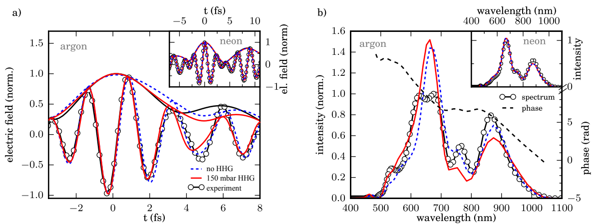
Figure 6.5: Signatures of pulse reshaping in the measured streaking field: Comparison of the experimentally measured laser waveforms (white dots with black solid line) to the simulated pulses for the case of 150 mbar pressure in the HHG target (red solid line) and the case with no high-harmonic generation (blue dashed line). Panels a) and b) show the comparison in the temporal domain and spectral domain, respectively. The main panels show the case of HHG in argon while the insets show the results for neon. In b), in addition to the spectral intensity, the spectral phase of the experimentally measured pulse is shown (black dashed line). The figure has been adapted from Ref. [29].
