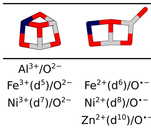
Figure 1. The two most relevant MAI_2O_4^+ isomers (aluminum: gray, oxygen: red) and their respective electron configurations for M=Al , Fe , Ni and Zn . While in the tricyclic cone-like structure (left) the metal site M^{3+} (dark blue) is found to be trivalent, it is reduced to M^{2+} in the ladder-like isomer (right) resulting in a terminal oxygen radical.
