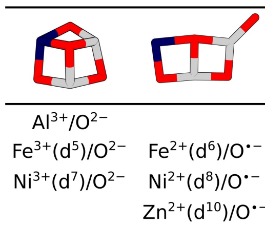
Figure 1. The two most relevant MAI_2O_4^+ isomers (aluminum: gray, oxygen: red) and their respective electron configurations for M=Al , Fe, Ni and Zn. While in the tricyclic cone-like structure (left) the metal site M^{3+} (dark blue) is found to be trivalent, it is reduced to M^{2+} in the ladder-like isomer (right) resulting in a terminal oxygen radical.
