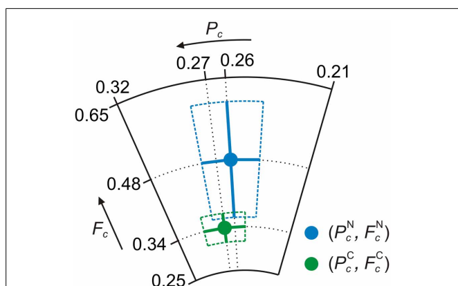
FIGURE 6 | Argand diagram of the NIXSW experimental results for AB/Ag(111). Green filled circle: Average experimental (P_c, F_c) = (0.27 \pm 0.02, 0.34 \pm 0.03) of carbon. Blue filled circle: Average experimental (P_c, F_c) = (0.26 \pm 0.02, 0.48 \pm 0.12) of nitrogen. Green and blue solid lines: Corresponding error bars. Green and blue dashed lines: Corresponding error regions [34].
