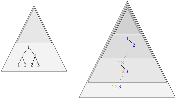
Figure 4: Left: Illustration of the tree automaton \mathcal{T} , tracking the number of right directions modulo n . Right: A path on which the runs of \mathcal{T} are disjoint.
