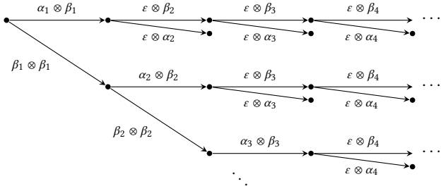
Figure 2: If v is a comb of the form v_i = \beta_1 \dots \beta_{i-1} \alpha_i then the convolutions v_i \otimes v_j for all i < j form a comb of combs.
