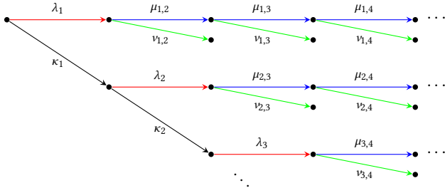
Figure 3: One can always find an infinite comb clique v with accepting runs which can be decomposed in the form \rho(v_i, v_j) = \kappa_1 \dots \kappa_{i-1} \lambda_i \mu_{i,i+1} \dots \mu_{i,j-1} v_{i,j} .
