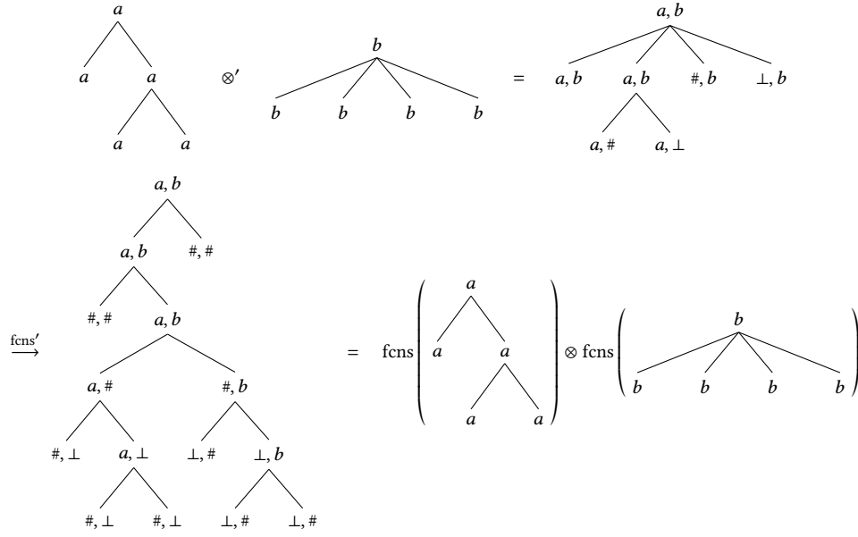
Figure 6: Example for adapted convolution and encoding
