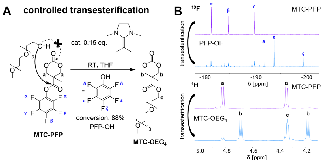
Figure 2. NHO-catalyzed transesterification of active ester carbonate monomer 5-methyl-5-pentafluorophenyl-oxycarbonyl-1,3-dioxane-2-one (MTC-PFP) by side chain reaction with alcohols. (A) Under the conditions of the controlled ROP for MTC-OBn, a polymerization does not occur. However, selective transesterification is observed and exploited for the synthesis of ester functional monomers (tetraethylene glycol monomethyl ether). (B) 19 F NMR spectra (top) showing high conversion of 88% by declining PFP ester signals ( \alpha , \beta , \gamma ) and rising signals of released PFP-OH ( \delta , \epsilon , \zeta ). 1 H NMR spectra (bottom) underlining the formation of the tetraethylene glycol ester product by a shift of the methylene signals from a (educt) to b (product) and the occurrence of alpha methylene protons by the formed ester c.
