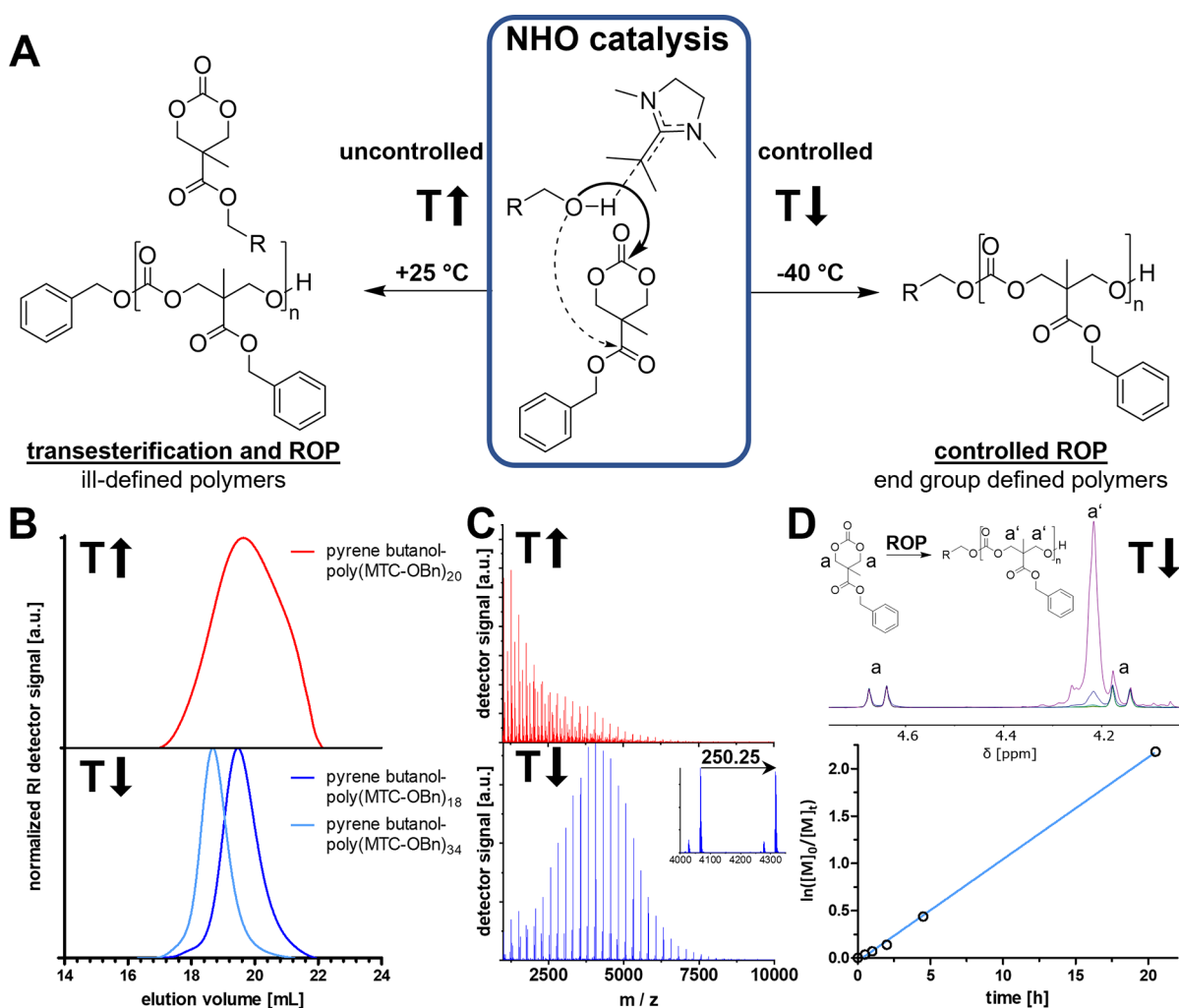
Figure 1. N -Heterocyclic olefins (NHO) as ring-opening polymerization (ROP) catalysts for functional six-membered carbonate 5-methyl-5-benzoyloxycarbonyl-1,3-dioxan-2-one (MTC-OBn). (A) Temperature-dependent tuning of catalyst activity from ROP and simultaneous transesterification at room temperature (RT, +25 °C) to selective ROP without side reactions at decreased temperatures (−40 °C). (B) SEC traces of homopolymers initiated by pyrene butanol showing broad distribution at RT (red trace) and narrow distributions at −40 °C (blue traces), recorded via refractive index (RI). (C) Mass spectrometric analysis of pyrene butanol-poly(MTC-OBn) 20 . Reactions at RT (red) provide various side products and a broad distribution compared to ROP at −40 °C with defined end groups (blue). Species deriving from two different ionization mechanisms were identified (photoionization with smaller intensities and K + cationization with larger intensities) with steps of 250.25 m/z (corresponding to the monomer mass of MTC-OBn). (D) Kinetic evaluation of controlled ROP of MTC-OBn at −40 °C targeting a DP of 40. Monitoring the conversion by 1 H NMR spectroscopy (top graph) with steady growth of polymer signal (a') and simultaneous decline of monomeric signal (a) reaching by conversion of 88.7%. Kinetic plot of conversion (bottom graph) as analyzed by 1 H NMR spectroscopy with linear reaction kinetics of pseudo-first-order, thereby providing controlled reaction propagation ( y = 0.1055 \cdot h^{-1} \cdot x , R^2 = 0.998 ).
