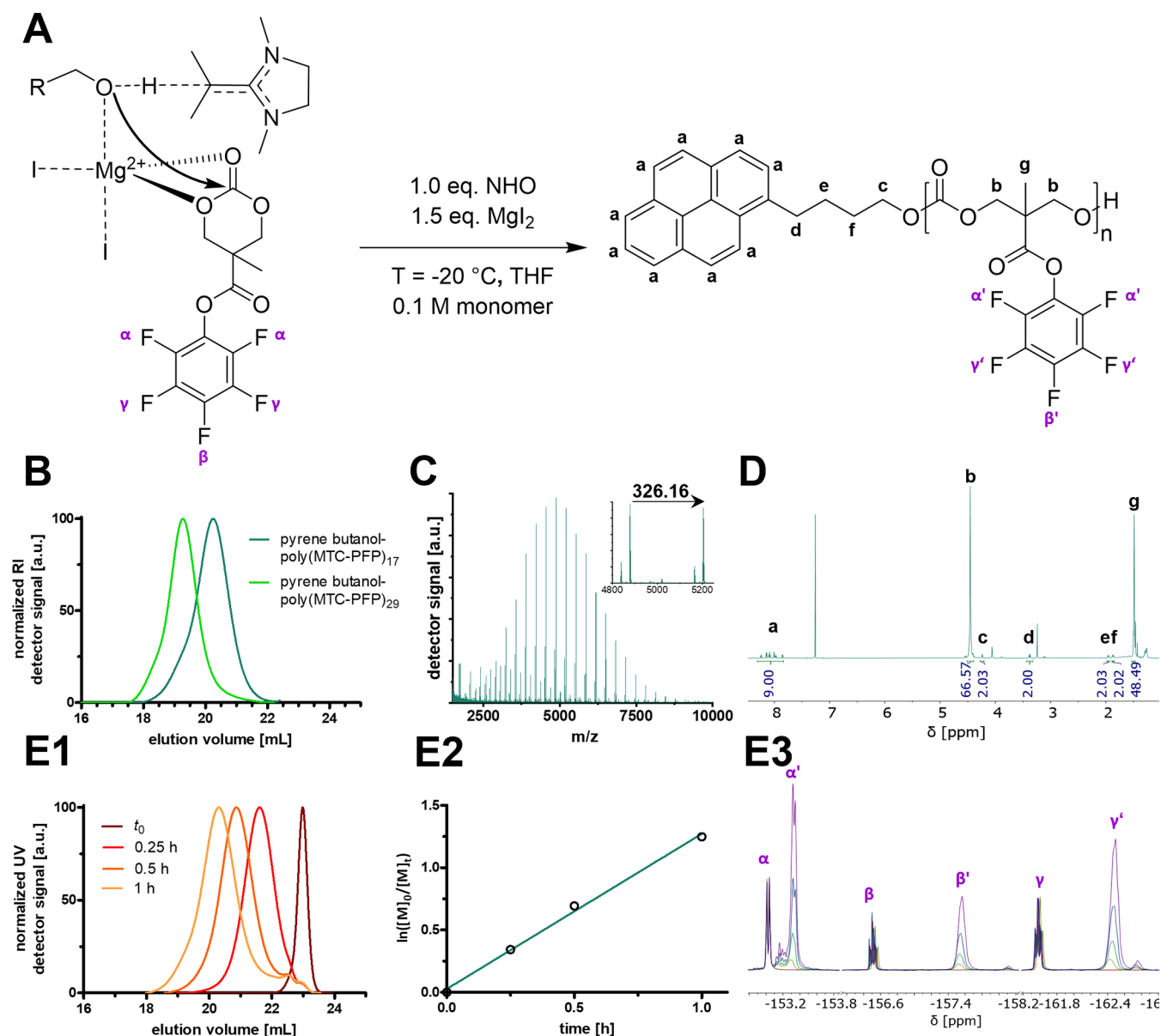
Figure 3. Controlled ROP of reactive ester monomer MTC-PFP by cocatalysis using NHO and Lewis acid magnesium iodide. (A) Proposed catalysis mechanism: By cooperative action by NHO and coordination by \text{MgI}_2 , propagating chain ends are directed toward ROP instead of transesterification. (B) SEC traces of homopolymers initiated at -20\text{ }^\circ\text{C} by pyrene butanol with narrow distributions recorded by refractive index (RI). (C) Mass spectrometric analysis of pyrene butanol-poly(MTC-PFP) 17 showing the high definition of cocatalyzed ROP at -20\text{ }^\circ\text{C} yielding polymers with defined end groups (green). Species deriving from two different ionization mechanisms were identified (photoionization, smaller intensity, and \text{K}^+ cationization, larger intensity) with steps of 326.16\text{ }m/z (corresponding to the monomer mass of MTC-PFP). (D) ^1\text{H} NMR spectrum of pyrene butanol-poly(MTC-PFP) 17 homopolymer. (E) Kinetic evaluation of controlled ROP of MTC-PFP at -20\text{ }^\circ\text{C} targeting a DP of 20. (E1) SEC analysis (UV detector) of MTC-PFP polymerization at various time points. (E2) Kinetic plot of conversion analyzed by ^{19}\text{F} NMR spectroscopy providing linear reaction kinetics of pseudo-first-order, thereby providing controlled reaction propagation ( y = 1.2805 \cdot \text{h}^{-1} \cdot x , R^2 = 0.998 ). (E3) Monitoring the conversion by ^{19}\text{F} NMR spectroscopy with steady growth of polymer signals ( \alpha' , \beta' , \gamma' ) and simultaneous decline of monomeric signals ( \alpha , \beta , \gamma ) reaching monomer conversion of \sim 80\% after 2 h.
