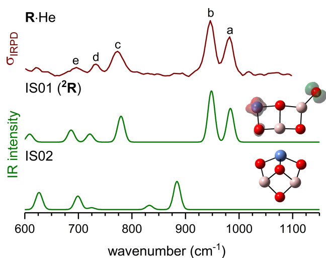
Figure 3. Experimental IRPD spectrum (dark red) of helium-tagged \text{NiAl}_2\text{O}_4^+ ( \text{R}\cdot\text{He} ). See Table S1 for positions and assignments of peaks a–e. Unscaled harmonic DFT (B3P86/TZVP) IR spectra (green), convolved using a Gaussian line shape function with a full-width-at-half-maximum of 15\text{ cm}^{-1} , and minimum-energy structures (blue, Ni; pink, Al; red, O) of the two lowest energy isomers IS01 ( ^2\text{R} ) and IS02 of \text{NiAl}_2\text{O}_4^+ in its doublet state (see Figure S4 for additional information on low energy isomers). For the IS01 ( ^2\text{R} ) structure, the spin distribution is shown; green indicates \beta -electron excess, red indicates \alpha -electron excess.
