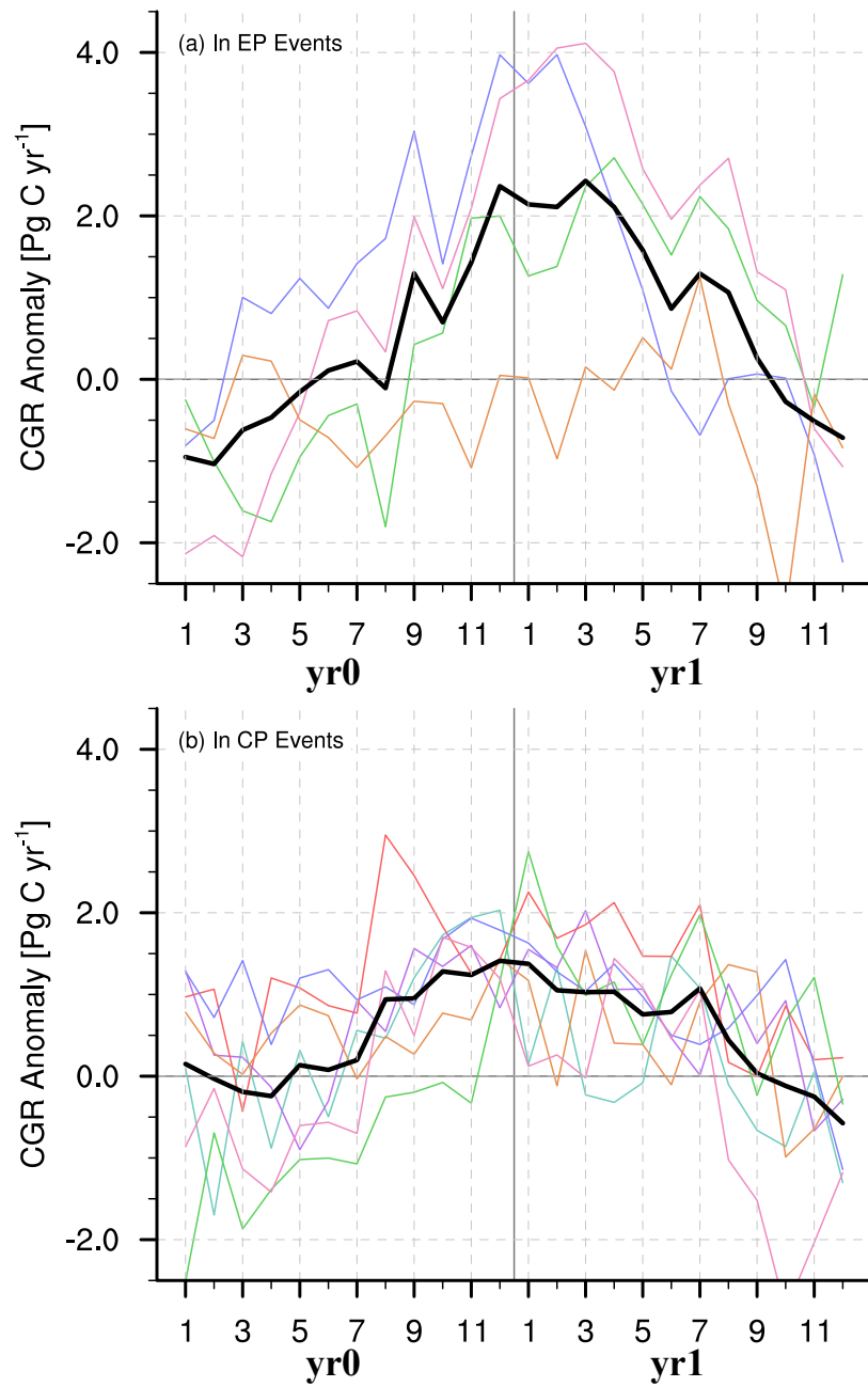
Figure S2 Behaviors of CGR anomalies ( \text{Pg C yr}^{-1} ) in the individual EP and CP El Niño events. (a) In EP Events. (b) In CP Events. The thickened black line represents the composite result.
