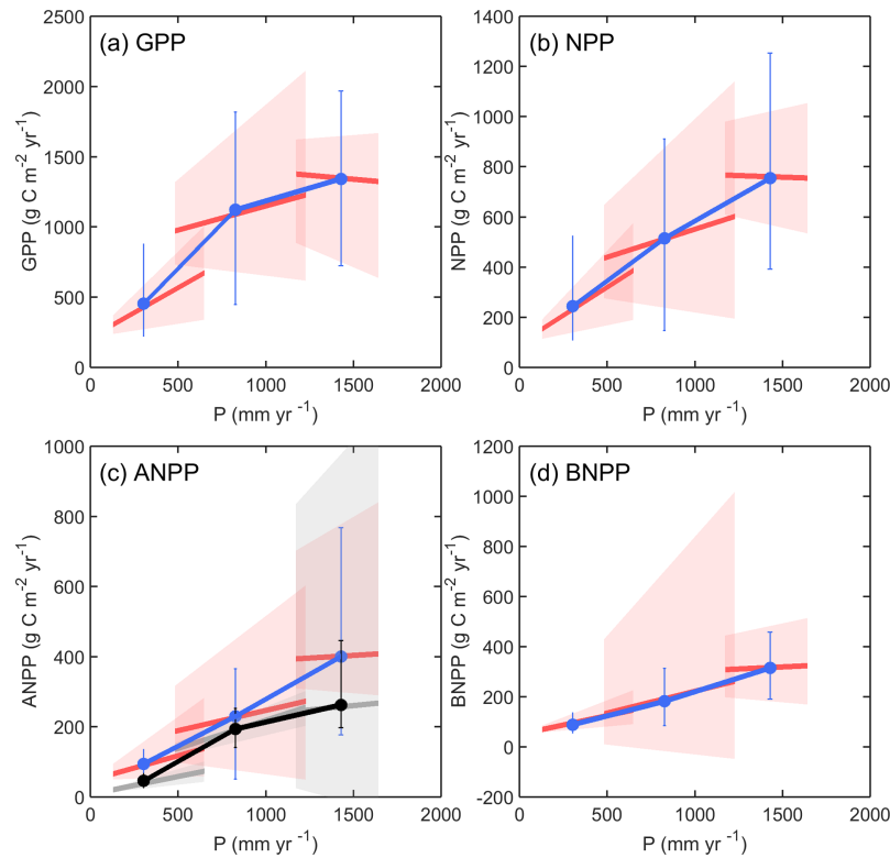
Figure 1. Relationships between GPP (a), NPP (b), ANPP (c), and BNPP (d) and precipitation ( P ) derived from multi-year ambient simulations (SC1) in two ways. Temporal slopes are site based and relate inter-annual variability in P to inter-annual variability in the productivities using linear regression analysis. Spatial slopes relate mean annual P to mean annual productivity across three sites. In each panel, SGS, KNZ and STU are from dry to moist, given from left to right. The red lines are the ensemble mean of modeled temporal slopes, and the red shading represents the model uncertainty range using the interquartile spread of the temporal slopes between individual simulations (10th and 90th percentiles). The blue line is the ensemble mean of modeled productivities, and the blue error bar represents the model uncertainty range using the interquartile spread of the productivities between individual simulations (10th and 90th percentiles). In (c), the grey lines are the observed temporal slopes, and the black line shows the observed spatial slope. The grey shading represents the observed uncertainty range using the bootstrap sampling method (10th and 90th percentiles), and the black error bar represents the observed uncertainty range using the interquartile spread of the inter-annual productivities (10th and 90th percentiles). Note that we simply converted observed ANPP from dry mass ( \text{g DM m}^{-2} \text{yr}^{-1} ) to carbon mass ( \text{g C m}^{-2} \text{yr}^{-1} ) with a factor of 0.5.
