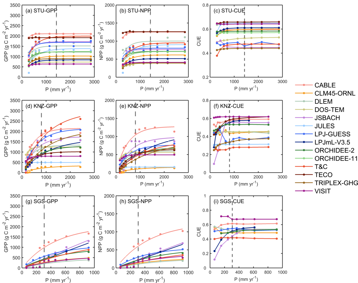
Figure 4. Responses of simulated annual GPP (a, d, g), NPP (b, e, h) and CUE (NPP/GPP; c, f, i) to altered and ambient precipitation ( P ) levels at the three sites STU, KNZ and SGS. The fitted equation is Eq. (8) for GPP and NPP (see Fig. S3 for fitted a and b ). The grey dashed line represents ambient precipitation. It should be noted that the x -axis scales are different between the sites.
