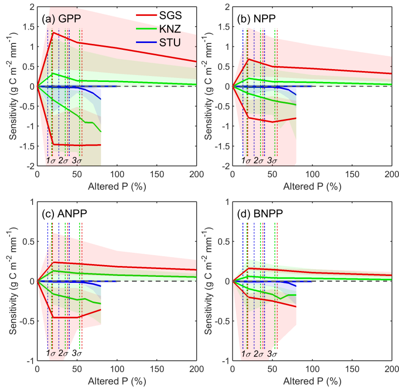
Figure 3. Sensitivity of GPP (a), NPP (b), ANPP (c) and BNPP (d) for altered precipitation simulations at the three sites SGS, KNZ and STU. Curves show the ensemble mean of models, and the shading represents the model uncertainty range using the interquartile spread of the sensitivities between individual simulations (10th and 90th percentiles). Curves above the zero line represent responses under increasing precipitation conditions relative to the control, and curves below the zero line show responses under decreasing precipitation conditions relative to the control. Vertical dashed lines represent precipitation variations of 1 standard deviation ( 1\sigma ), 2 standard deviations ( 2\sigma ) and 3 standard deviations ( 3\sigma ), which were derived from long-term annual precipitation at the three sites respectively.
