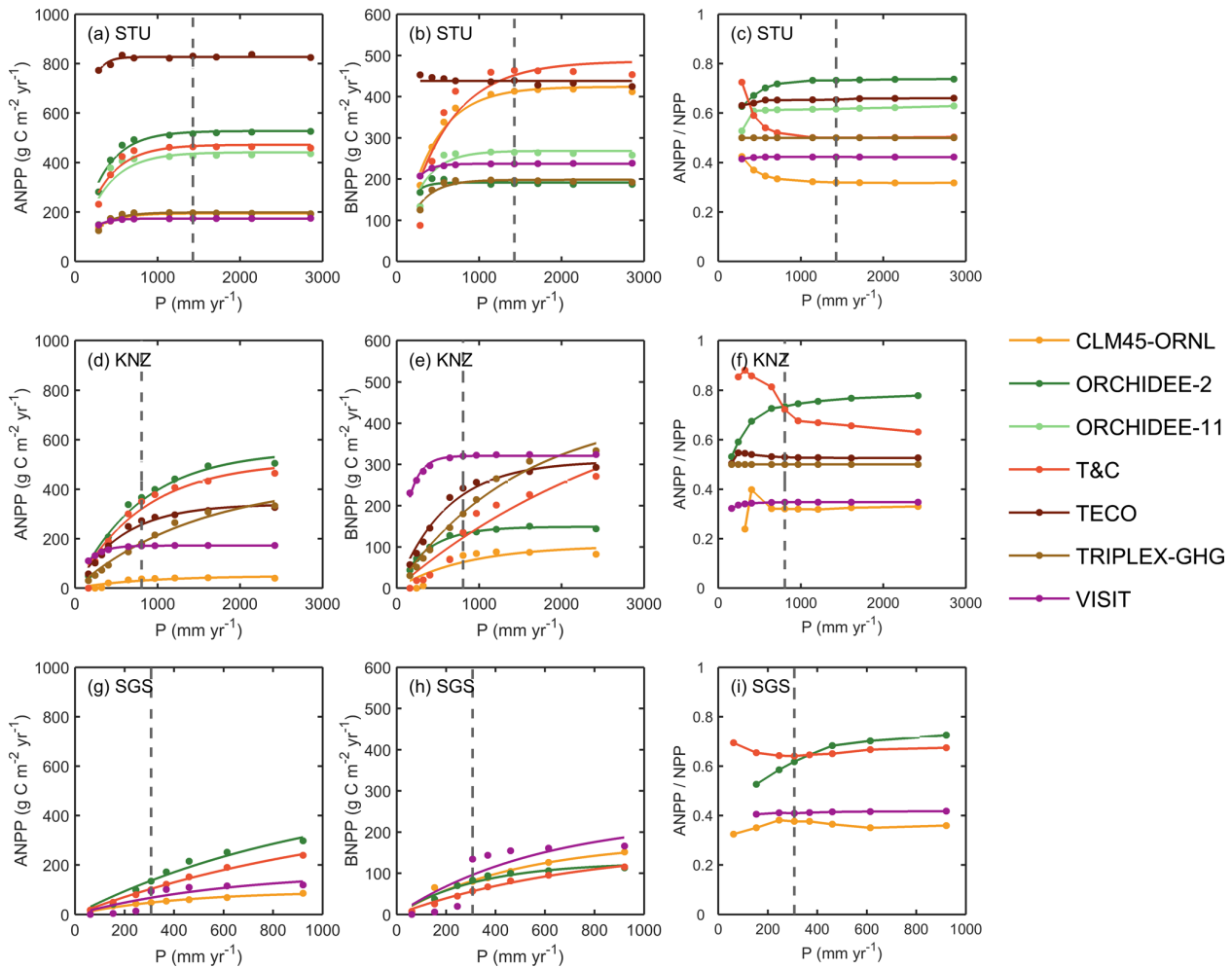
Figure 5. Responses of simulated annual ANPP (a, d, g), BNPP (b, e, h), and the ratio of ANPP and NPP (c, f, i) to altered and ambient precipitation ( P ) levels at the three sites STU, KNZ and SGS. The fitted equation is Eq. (8) for ANPP and BNPP (see Fig. S4 for fitted a and b ). The grey dashed line represents ambient precipitation. It should be noted that the x -axis scales are different between the sites.
