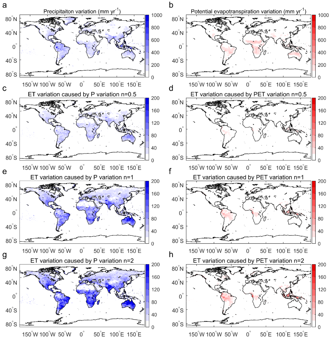
Fig. S15. The spatial pattern of precipitation variation from GPCP and PET variation from MODIS MOD16, both datasets are annual sums from 2000-2013 (a, b). ET variation caused by precipitation variation and by PET variation with different n values (c - h). Maps were created using Matlab R2016a ( http://www.mathworks.com/products/matlab/ ).
