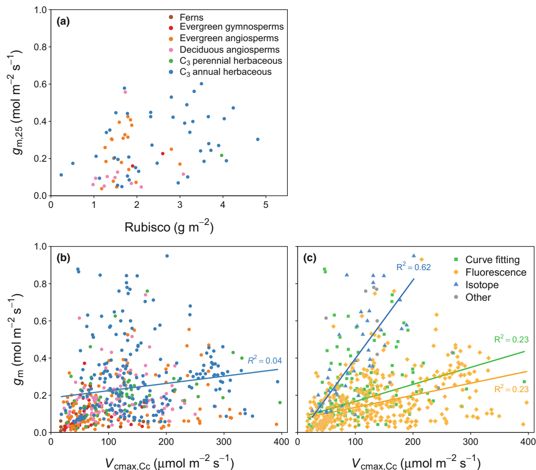
Fig. 5 Relationship between mesophyll conductance standardised to 25°C ( g_{m,25} ) and (a) leaf Rubisco content, (b) maximum carboxylation rate derived from A_n - C_c curves ( V_{\text{max,Cc}} ) and (c) same as (b) but data grouped by the measurement method applied. g_m and V_{\text{max,Cc}} in panels (b, c) were measured at the same temperature. Lines represent robust linear regression fits and were drawn if P < 0.05 .
