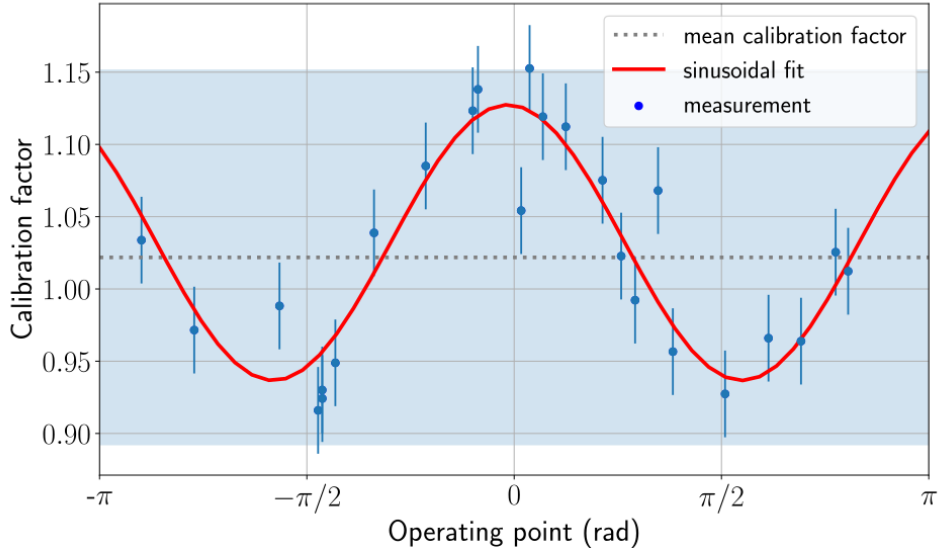
Figure 7. Measured nonlinear dependence of the calibration on the operating point of the HoQI (blue dots). The error bars are set by the deviations occurring between averages in the measurement. The data points are fitted (solid red) to a function given in eq. (10). In the measurement, deviations of up to 13% from the mean calibration occurred (blue-shaded area).
