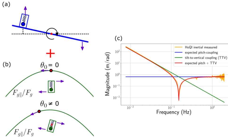
Figure 6. The total coupling of table tilt into the sensor signal (red) is the sum of a (a) position-based coupling (blue) and (b) tilt-to-vertical coupling (green), the latter scaling with the sensor’s angular misalignment \theta_0 with respect to gravity. (c) shows the transfer function for vertical inertial motion measured with the HoQI for pitch actuation (orange). It is reproducible from the expected position-based, frequency independent pitch coupling (blue) and tilt-to-vertical coupling (green).
