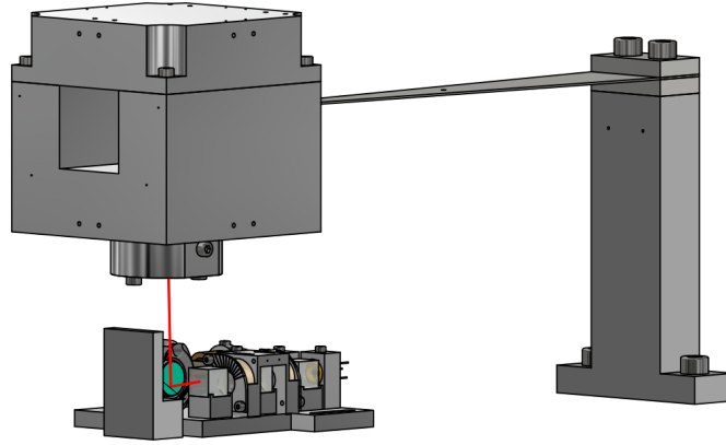
Figure 2. A possible redesign for the sensor with a total mass of 1.75 kg.
