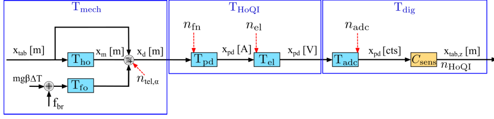
Figure 3. Block diagram of the HoQI-based inertial sensor including transfer functions of individual components T_i , signals x_i and noise contributions n_i . The photodiode response T_{pd} , transfer functions of the readout electronics T_{el} and the analogue-to-digital converter T_{adc} are frequency-independent in the frequency band of interest. The block C_{sens} represents the mathematical functions applied digitally to the three photodiode signals to calculate the optical phase of the interferometer.
