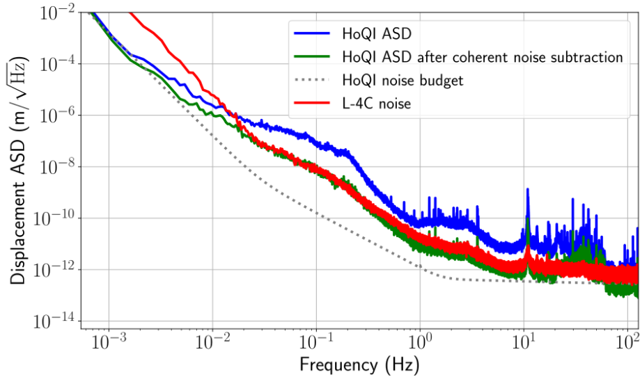
Figure 5. Result of a huddle test for the novel vertical inertial sensor carried out in vacuum using a seismically isolated platform.
