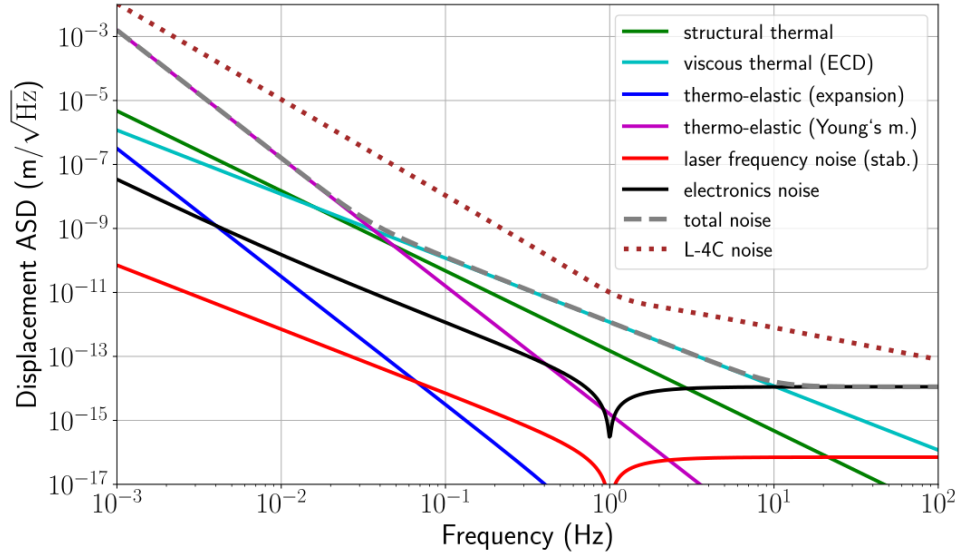
Figure 4. Modeled noise budget for the novel vertical inertial sensor depicted as displacement amplitude spectral density (ASD). The total sensor noise (dashed grey) is modeled to be dominated by thermoelastic noise due to temperature-induced change in Young’s modulus below 30 mHz (solid purple), by viscous thermal noise due to eddy current damping (ECD) between 30 mHz and 10 Hz (solid cyan).
