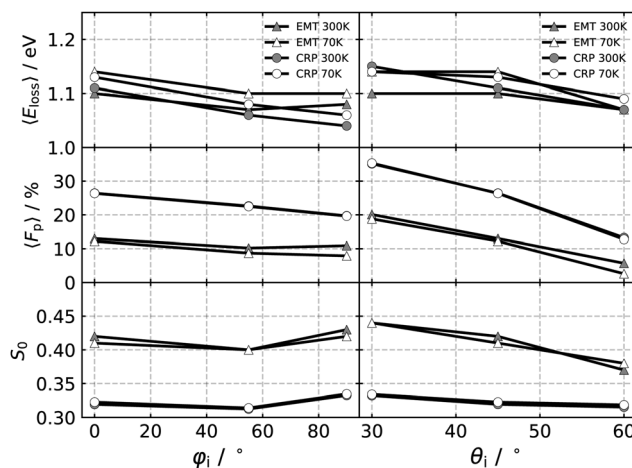
Fig. 5 Mean energy loss ( \langle E_{\text{loss}} \rangle ), fraction of scattered particles after penetration into the surface F_p and sticking coefficient S_0 as a function \varphi_i with \theta_i = 45^\circ (left) for E_c = 2.76 eV. Same quantities as a function of \theta_i with \varphi_i = 0^\circ (right). \langle E_{\text{loss}} \rangle and F_p were calculated from all scattering events.
