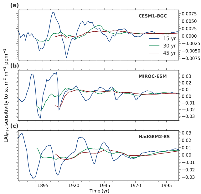
Figure 4. Temporal variation of LAI_{\max} sensitivity to \omega in three selected CMIP5 models spanning the full range from low-end (CESM1-BGC, a), to closest to observations (MIROC-ESM, b), to high-end (HadGEM2-ES, c). The colored lines show LAI_{\max} sensitivity variations for moving windows of varying length: 15 (blue), 30 (green), and 45 (red) years over the historical period from 1860 to 2005.
