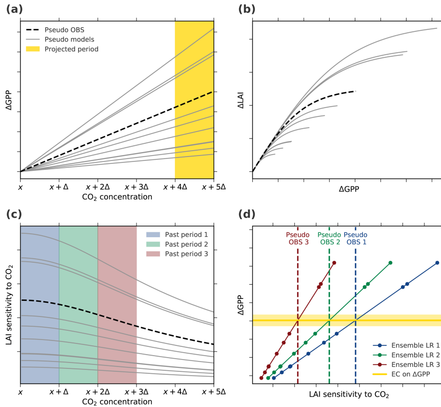
Figure 6. Thought experiment to examine the applicability of EC analysis under the assumption of an idealized linear–nonlinear behavior of the system (Case 3, Table A1). (a) Changes in GPP relate linearly to changes in CO 2 concentration. The yellow band marks the projection period of interest, i.e., the period of CO 2 concentration from x + 4\Delta to x + 5\Delta . (b) The increment in LAI with increasing GPP is assumed to decrease with rising CO 2 concentration (described by a hyperbolic tangent function). The parameterization in the linear and nonlinear functions for pseudo observations (dashed black line) as well as models (solid gray lines) is determined randomly for each model. (c) The diagnostic variable, LAI sensitivity to CO 2 , decreases with increasing CO 2 as a consequence of the nonlinear relation between \Delta GPP and \Delta LAI. The colored bands indicate three “past” periods from x to x + \Delta (blue), x + \Delta to x + 2\Delta (green), and x + 2\Delta to x + 3\Delta (red). (d) Linear relationships among the pseudo model ensembles (Ensemble LR, colored lines) between LAI sensitivities to CO 2 of the three past periods and \Delta GPP from the projected period. Colored dots mark different models and the dashed lines represent associated pseudo observations for the respective historical period. The solid yellow line depicts the constant EC on projected \Delta GPP irrespective of the past period.
