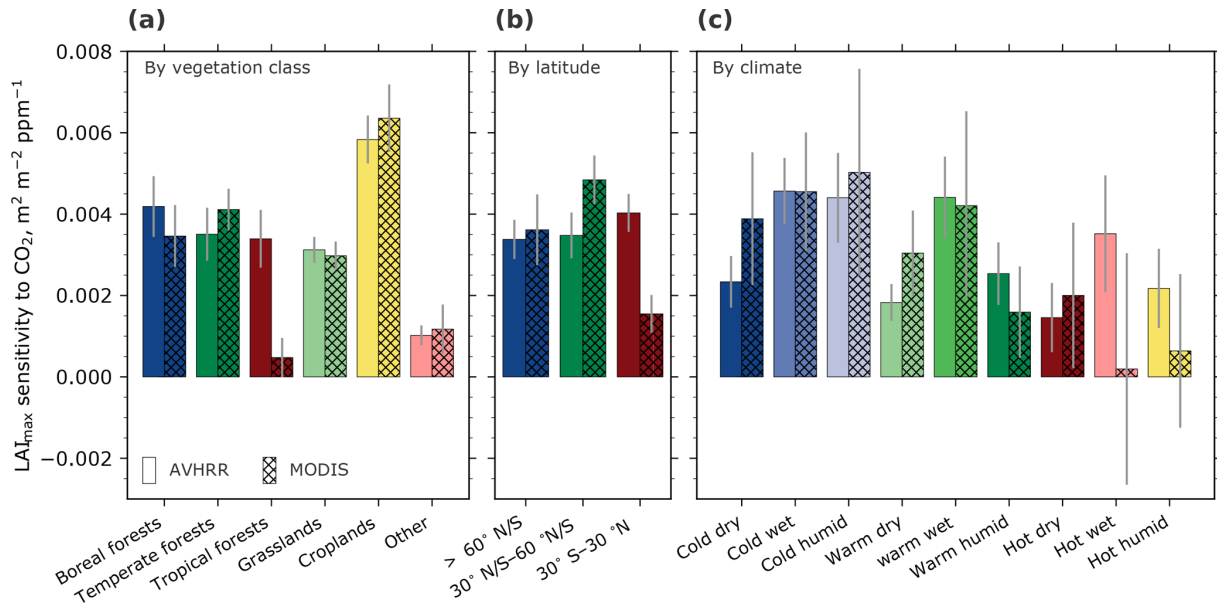
Figure 2. Bar charts showing regression slopes of LAI_{max} against atmospheric CO_2 concentration for broad vegetation classes (a) (Olson et al., 2001; Fritz et al., 2015), latitudinal bands (b), and climate regimes (c). The class “Other” includes deserts, mangroves, barren and urban land, snow and ice, and permanent wetlands. The climatic boundaries are defined as follows: cold: < 10^\circ C ; warm: > 10 and < 25^\circ C ; hot: > 25^\circ C ; dry: < 500 \text{ mm a}^{-1} ; wet: > 500 and < 1000 \text{ mm a}^{-1} ; humid: > 1000 \text{ mm a}^{-1} . Sensitivities evaluated from data from two satellite-borne sensors are shown, AVHRR (1982–2016; Pinzon and Tucker, 2014) and MODIS (2000–2016; Yan et al., 2016a, b). Gray bars indicate the standard error of the best linear fit.
