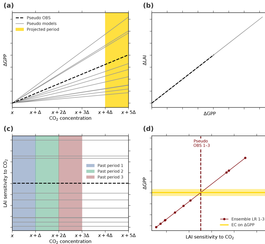
Figure A5. Thought experiment to examine the applicability of the EC analysis assuming an idealized linear–linear behavior of the system (Case 1, Table A1). (a) Changes in GPP relate linearly to changes in \text{CO}_2 concentration. The yellow band marks the projection period of interest, i.e., the period of \text{CO}_2 concentration from x + 4\Delta to x + 5\Delta . (b) Changes in LAI relate linearly to changes in GPP. The parameterization in the linear functions for pseudo observations (dashed black line) as well as models (solid gray lines) is determined randomly for each model. (c) The diagnostic variable, LAI sensitivity to \text{CO}_2 , remains constant with increasing \text{CO}_2 as a consequence of the overall linear characteristics of the system. The colored bands indicate three “past” periods from x to x + \Delta (blue), x + \Delta to x + 2\Delta (green), and x + 2\Delta to x + 3\Delta (red). (d) Linear relationships among the pseudo model ensembles (Ensemble LR 1–3 on top of each other, red) between LAI sensitivity to \text{CO}_2 of the three past periods and \Delta\text{GPP} from the projected period. Red dots mark different models and the dashed line represents associated pseudo observations for all three historical periods. The solid yellow line depicts the constant EC on projected \Delta\text{GPP} irrespective of the past period.
