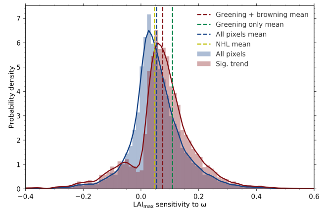
Figure 3. Histograms and associated probability density functions (Gaussian kernel density estimation) of observed \text{LAI}_{\text{max}} sensitivity to \omega at pixel scale for the northern high-latitude band ( > 60^\circ \text{N} , data from AVHRR sensor). Blue depicts the distribution of \text{LAI}_{\text{max}} sensitivities of all pixels and red is for pixels with statistically significant (Mann–Kendall test, p < 0.1 ) greening or browning trends (the dashed lines denote the respective mean value). The green dashed line shows the mean value of “greening” pixels only, whereas the dashed yellow line shows the \text{LAI}_{\text{max}} sensitivity to \omega for the entire northern high-latitude belt.
