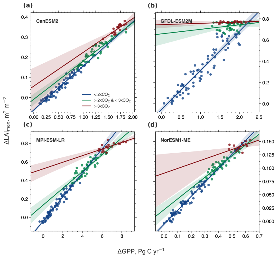
Figure A4. Correlation of \Delta\text{LAI}_{\text{max}} and \Delta\text{GPP} with increasing \text{CO}_2 forcing, starting from a preindustrial concentration of 280 \text{ ppm} ( 1 \times \text{CO}_2 ) to 4 \times \text{CO}_2 (CMIP5 1pctCO2 simulations). Results are shown for four CMIP5 models analogous to Fig. 5. Blue colored dots show the relation between 1 \times \text{CO}_2 and 2 \times \text{CO}_2 , green colored dots between 2 \times \text{CO}_2 and 3 \times \text{CO}_2 , and red colored dots between 3 \times \text{CO}_2 and 4 \times \text{CO}_2 . The respective colored lines represent the best linear fit through those dots and the shading represents the 95 % confidence interval.
