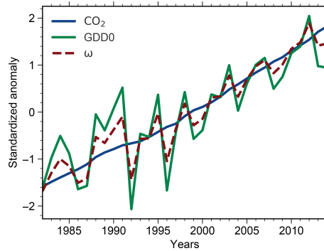
Figure A1. Standardized temporal anomalies of annual averaged atmospheric CO 2 concentration (blue solid line), area-weighted averaged GDD0 for NHLs (green solid line), and their leading principal component \omega (red dashed line) in observations.
