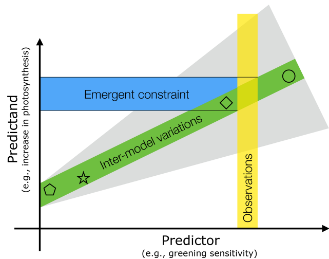
Figure 1. Schematic depiction of the emergent constraint (EC) method and factors affecting the uncertainty of the constrained estimate. The predictor ( x axis) is change in the annual maximum of green leaf area index ( LAI_{max} ) due to unit forcing ( CO_2 increase and associated climatic changes) during a representative historical period. It is termed greening sensitivity in this study. The predictand ( y axis) is projected change in gross primary productivity (GPP) in response to rising CO_2 concentration (e.g., for a doubling of the preindustrial level). Both the predictor and predictand refer to large area values: in this case, the entire northern high latitudes (NHLs). Inter-model variations (each symbol represents a model) in matching pairs of predictors and predictands result in a linear relationship between the two (green band); i.e., the ratio (predictand / predictor) is approximately constant across the model ensemble. The slope depends on forcing attributes (gray shading), such as its level ( CO_2 concentration; Sect. 3.4), time rate of application (scenarios such as various RCPs; Sect. 3.4), and different effects (i.e., fertilization, radiative forcing; Sect. 3.5). The observed sensitivity (vertical yellow bar) is used to find the constrained estimate of the predictand (i.e., change in GPP). The ability to accurately estimate the predictor depends on the source of observational data (Sect. 3.1) and its spatial (Sect. 3.2) and temporal variability (Sect. 3.3). Observed (yellow bar) and modeled predictor values ( x coordinate of symbols) must be obtained from matching time periods, i.e., at the same level of historical forcing, to ensure comparability (Sect. 3.3 and 3.4). All these factors, together with the goodness of fit of inter-model variations (width of green shading), finally define the uncertainty of the derived constrained estimate (blue horizontal bar with black solid lines depicting the upper and lower bound of uncertainty).
