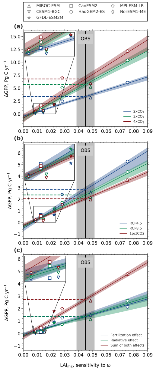
Figure 7. Linear relationships between the historical sensitivity of \text{LAI}_{\text{max}} to \omega and an absolute increase in GPP at different levels (a), different time rates (b), and the effects of rising CO 2 (c). The solid black line depicts the observational sensitivity including the standard error (gray shading). Each CMIP5 model is represented by a distinct marker (legend at the top). The colored lines show the best linear fits including the 68 % confidence interval estimated by bootstrapping across the model ensemble. The colored dashed lines indicate the derived constraints on \Delta\text{GPP} . (a) Absolute changes in GPP at different levels of CO 2 : 2 × CO 2 (blue), 3 × CO 2 (green), and 4 × CO 2 (red). (b) Absolute changes in GPP for a rising CO 2 concentration from 380 to 535 ppm at different time rates: RCP4.5 (90-year, blue), RCP8.5 (45-year, green), and 1pctCO 2 (30-year, red). (c) Absolute changes in GPP due to the two disentangled effects of CO 2 at 2 × CO 2 in idealized simulations: fertilization effect (esmFixClim1, blue), radiative effect (esmFdbk1, green), and the sum of both effects (red).
