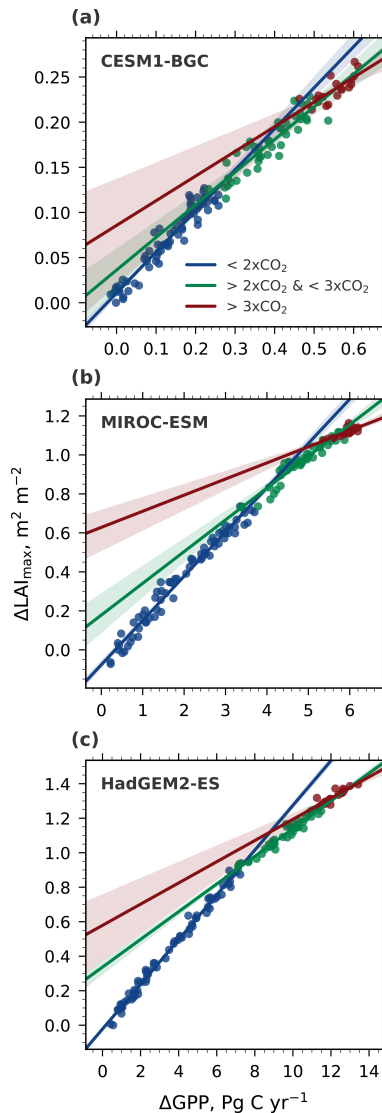
Figure 5. Correlation of \Delta\text{LAI}_{\text{max}} and \Delta\text{GPP} with increasing \text{CO}_2 forcing, starting from a preindustrial concentration of 280 ppm ( 1 \times \text{CO}_2 ) to 4 \times \text{CO}_2 (CMIP5 1pctCO2 simulations). Results are shown for three selected CMIP5 models spanning the full range of \text{LAI}_{\text{max}} sensitivity to \omega : low-end: CESM1-BGC (a), closest to observations: MIROC-ESM (b), and high-end: HadGEM2-ES (c). Blue colored dots show the relation between 1 \times \text{CO}_2 and 2 \times \text{CO}_2 , green colored dots between 2 \times \text{CO}_2 and 3 \times \text{CO}_2 , and red colored dots between 3 \times \text{CO}_2 and 4 \times \text{CO}_2 . The respective colored lines represent the best linear fit through those dots and the shading represents the 95 % confidence interval.
