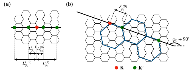
FIG. 7. Geometrical proof of the fractal property of the triangular lattice. (a) For a horizontal line (black) ( \varphi_0 = 90^\circ ) passing through the \mathbf{K} (red) and \mathbf{K}' (green) points, the zero-energy tunneling paths are given by L_{\varphi_0}^{(n)} = (3n + 1)L_{\varphi_0}^{(0)} . (b) For an arbitrary line with orientation \varphi_0 , the proof is identical to the case of \varphi_0 = 90^\circ . This is because the line passes through the corners of the larger unit cell (blue hexagons) of the reciprocal space similar as in (a).
