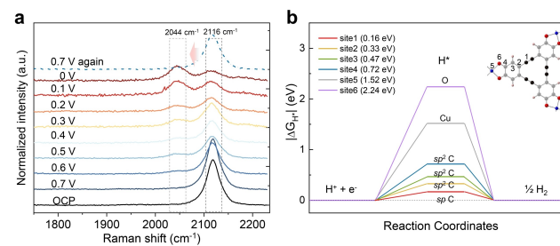
Figure 5. a) Potential-dependent Raman spectra of \text{Cu}_3\text{HHAE}_2 in 0.1 M \text{Na}_2\text{SO}_4 under 594 nm laser excitation (OCP, open circuit potential). Operando resonance Raman spectra. b) Free-energy diagram for \text{H}_2 -evolution via a single-site reaction pathway: 1, 2, 3, 4, 5, 6 denote different active sites of \text{Cu}_3\text{HHAE}_2 .
