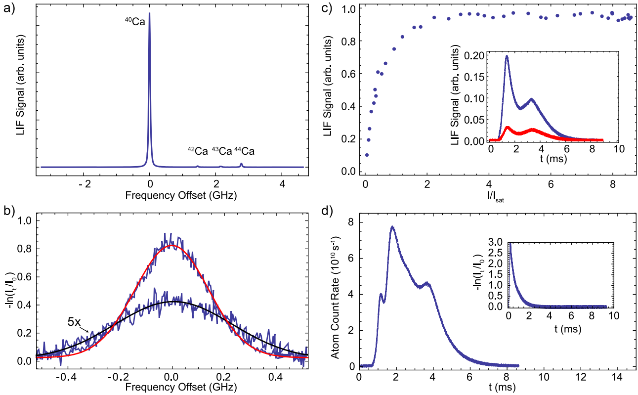
Figure 7. (a) LIF spectrum of the (3p^64snp)^1P_1 \leftarrow (3p^64s^2)^1S_0 line of Ca. The observed isotope peaks are labelled. (b) Absorption spectra of the (3p^64snp)^1P_1 \leftarrow (3p^64s^2)^1S_0 transition in ^{40}\text{Ca} , recorded directly outside the cell exit (Gaussian fit shown in red) and 20 mm downstream (black). (c) Fluorescence saturation curve of the (3p^64snp)^1P_1 \leftarrow (3p^64s^2)^1S_0 transition of Ca. The inset shows the LIF TOF without (blue) and with (red) a pumping laser tuned the same transition frequency. (d) Fluorescence and absorption TOF traces of the Ca beam, using light resonant with the (3p^64snp)^1P_1 \leftarrow (3p^64s^2)^1S_0 transition of ^{40}\text{Ca} .
