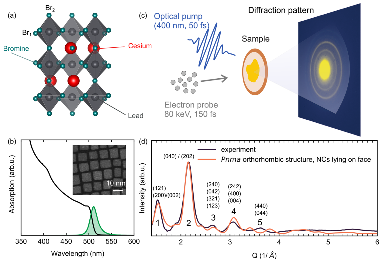
Figure 1. (a) Orthorhombic crystal structure of \text{CsPbBr}_3 from ref 44, with the two inequivalent bromine atoms labeled. (b) Linear absorption (plain black line) and photoluminescence (filled green) spectra of the \text{CsPbBr}_3 NCs dispersed in toluene. Inset: TEM picture showing the NCs in real space. (c) Schematic illustration of the FED experiment, with an example diffraction pattern of the NCs as collected by our detector. (d) Diffraction profile of the \text{CsPbBr}_3 NCs (dark line), obtained by azimuthally averaging the pattern shown in (c). An empirical function was employed to remove background contributions. The orange curve represents the simulated pattern using the structure from ref 44 and assuming the NCs lie flat on their faces.
